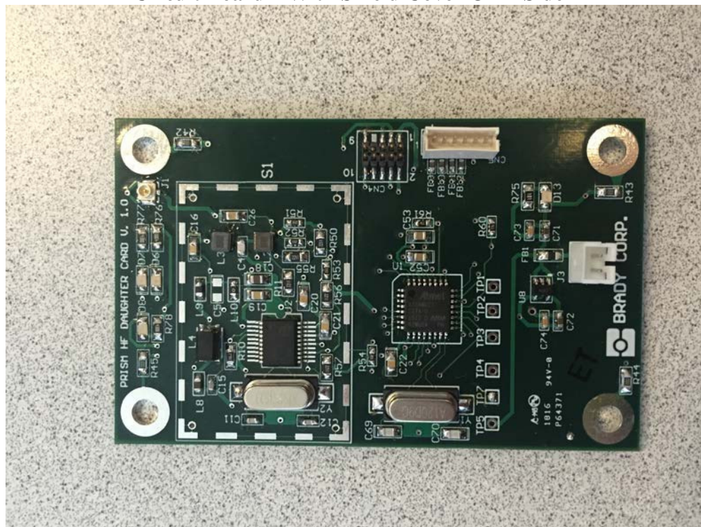
Circuit Board – With Shield Cover Off – Side 1
