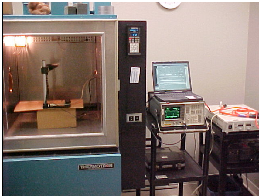
View of the EUT during the Frequency Stability testing
