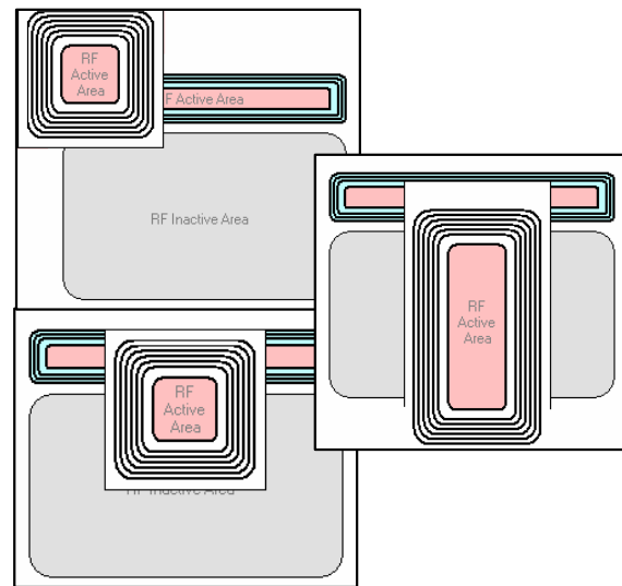
Figure 5-7 Bad XE2000 & Label Positioning
