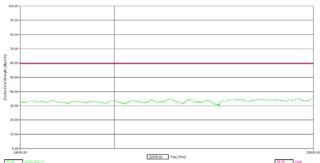
Figure 9: Radiated Emission (Average) – Horizontal polarization 18GHz to 25GHz – Bluetooth, Channel 0
