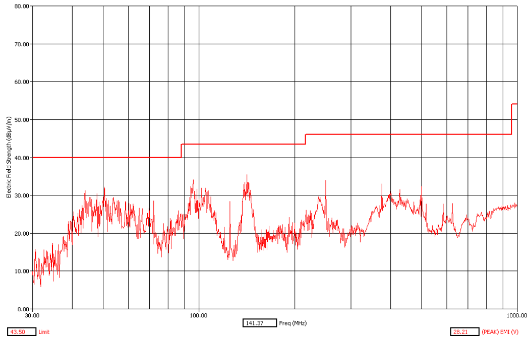
Figure 20: Radiated Emission (Peak) – Vertical polarization – 30 MHz to 1 GHz – Bluetooth, Channel 78
