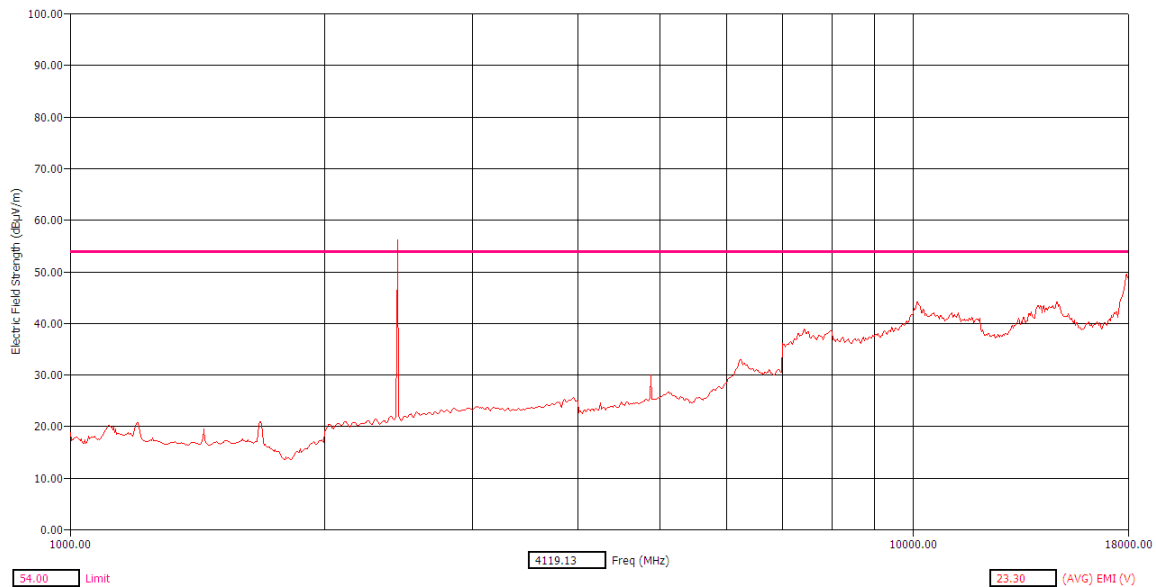
Figure 17: Radiated Emission (Average) – Vertical polarization – 1 GHz to 18 GHz – Bluetooth, Channel 40
