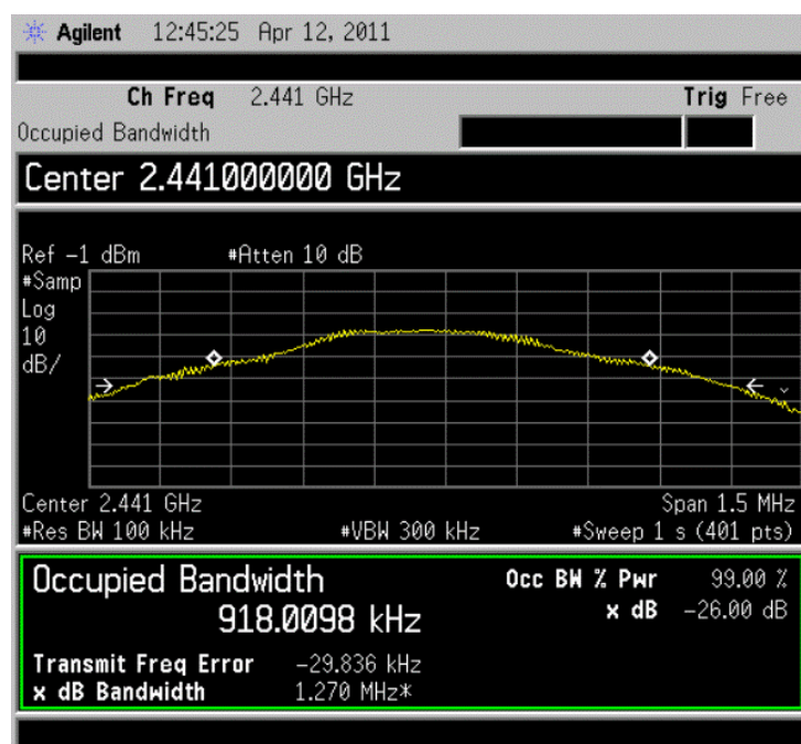
Figure 50: Occupied Bandwidth Measurement – Bluetooth, Mid channel (39)
