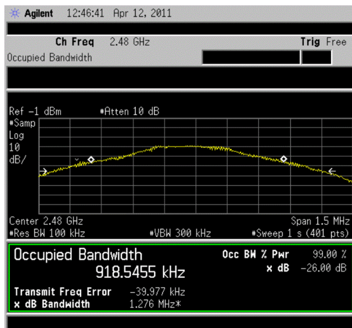
Figure 51: Occupied Bandwidth Measurement – Bluetooth, High channel (78)
