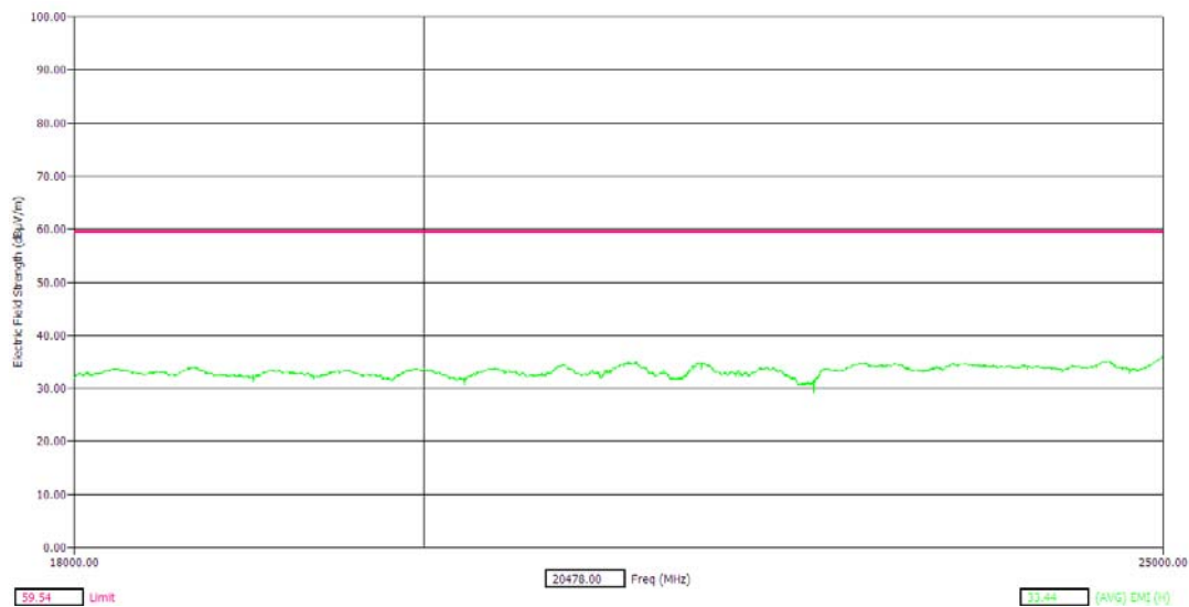
Figure 23: Radiated Emission (Average) – Horizontal polarization 18GHz to 25GHz – Bluetooth, Channel 78
