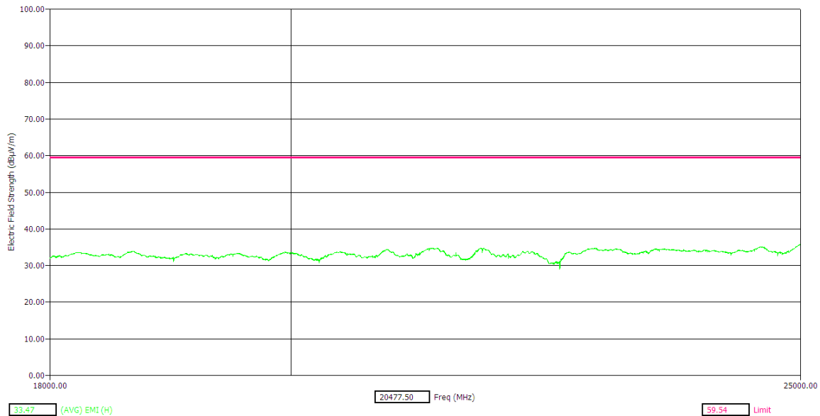
Figure 16: Radiated Emission (Average) – Horizontal polarization – 18GHz to 25GHz – Bluetooth, Channel 40
