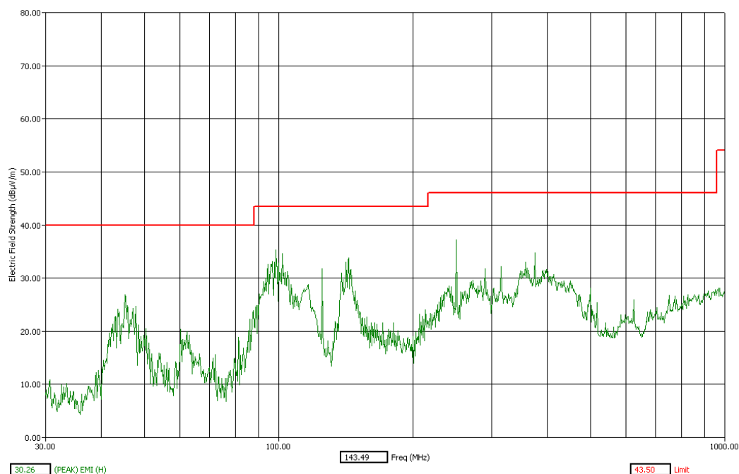
Figure 12: Radiated Emission (Peak) – Horizontal polarization – 30 MHz to 1 GHz – Bluetooth, Channel 40
