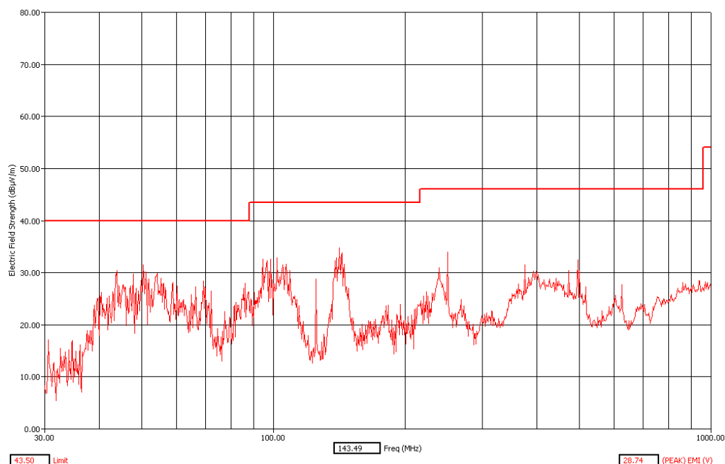
Figure 13: Radiated Emission (Peak) – Vertical polarization – 30 MHz to 1 GHz – Bluetooth, Channel 40
