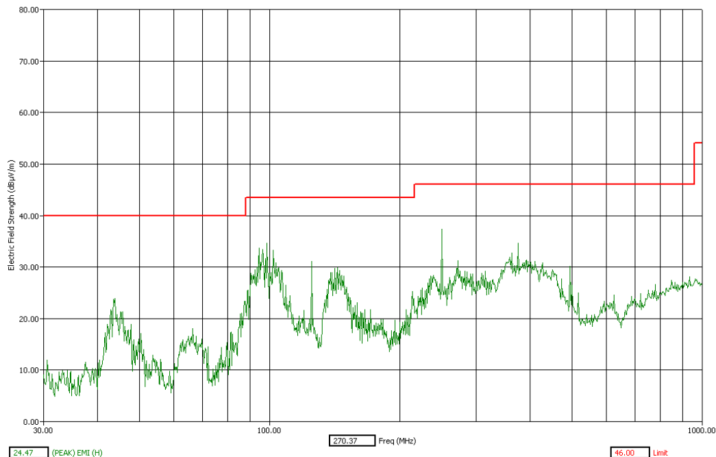
Figure 5: Radiated Emission (Peak) – Horizontal polarization – 30 MHz to 1 GHz – Bluetooth, Channel 0
