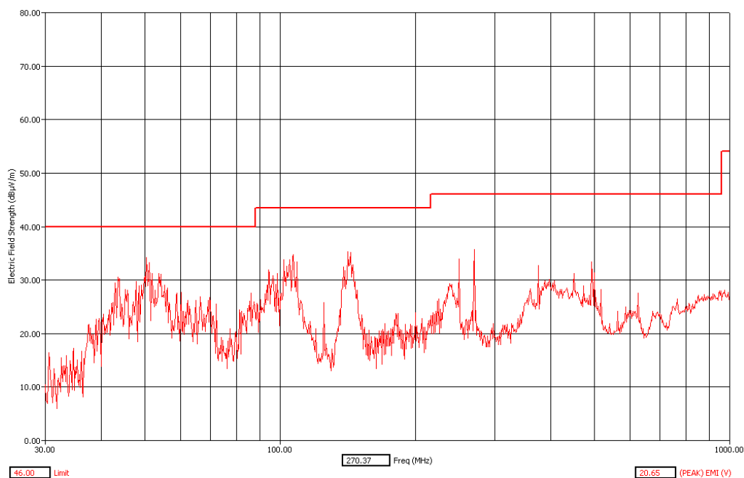
Figure 6: Radiated Emission (Peak) – Vertical polarization – 30 MHz to 1 GHz – Bluetooth, Channel 0
