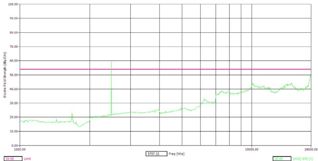
Figure 22: Radiated Emission (Average) – Horizontal polarization 1GHz to 18GHz – Bluetooth, Channel 78
