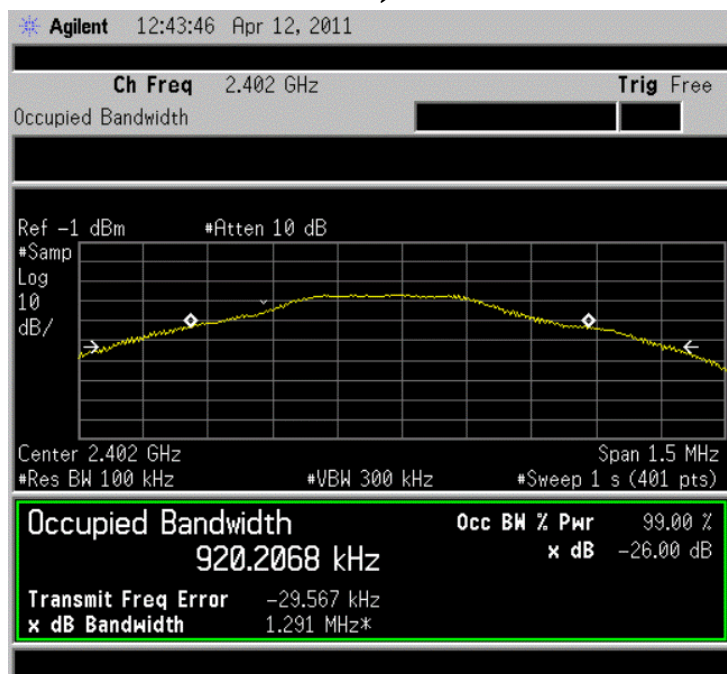
Figure 49: Occupied Bandwidth Measurement – Bluetooth channel (0)
