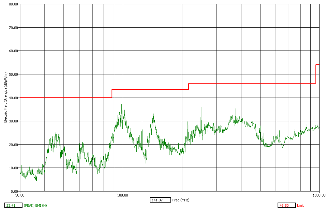
Figure 19: Radiated Emission (Peak) – Horizontal polarization – 30 MHz to 1 GHz – Bluetooth, Channel 78
