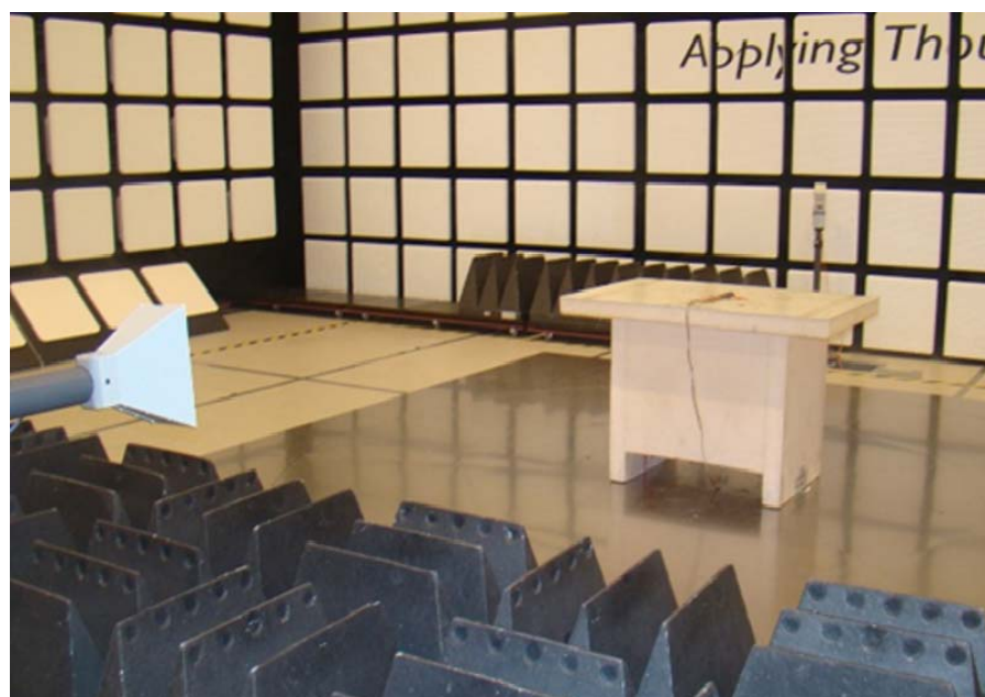
Figure 4: Test setup for Radiated Emission (Horizontal) – 1GHz to 18GHz
