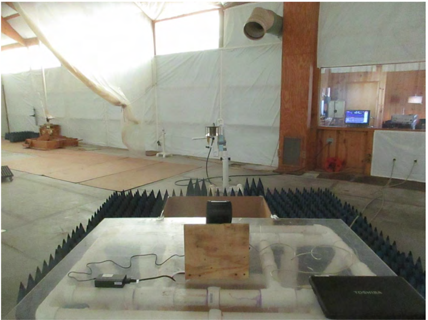
Radiated Emissions Above 1GHz Back
