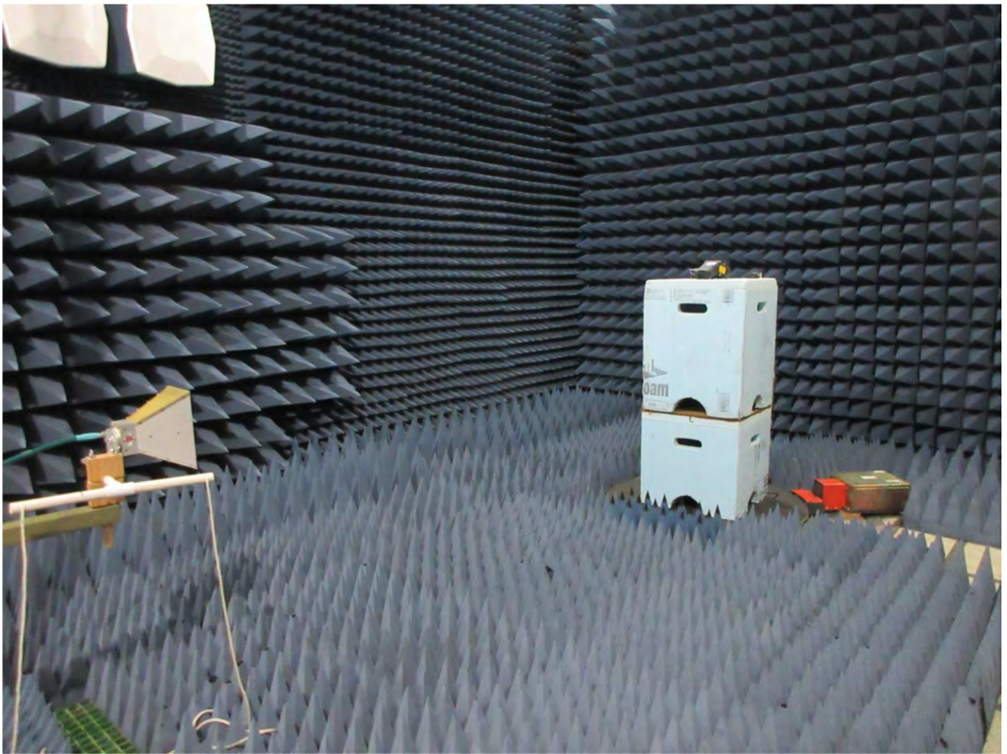
Radiated Emissions Above 1GHz BLE
