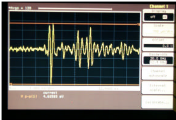
Fig.4.17: Line-of-sight waveform at 25 feet
