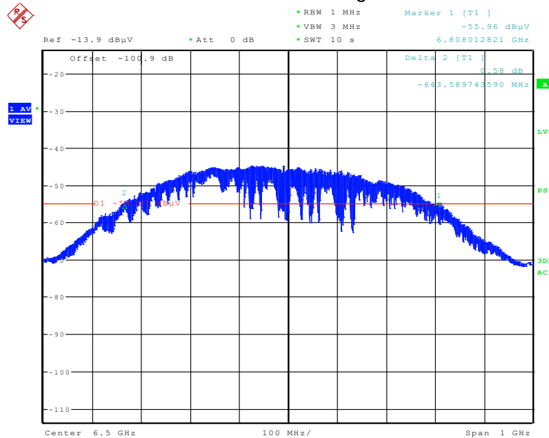
Bandwidth Plot – High Channel
