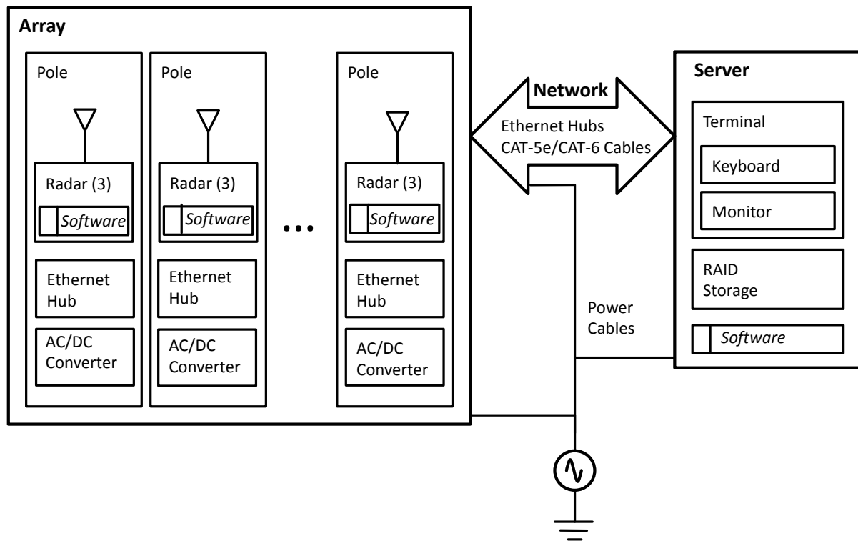
Figure 2 USS Hardware Components
