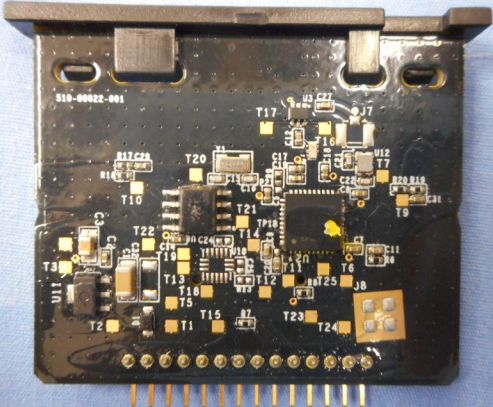
Internal Photo: Interior Lock Radio PCB
