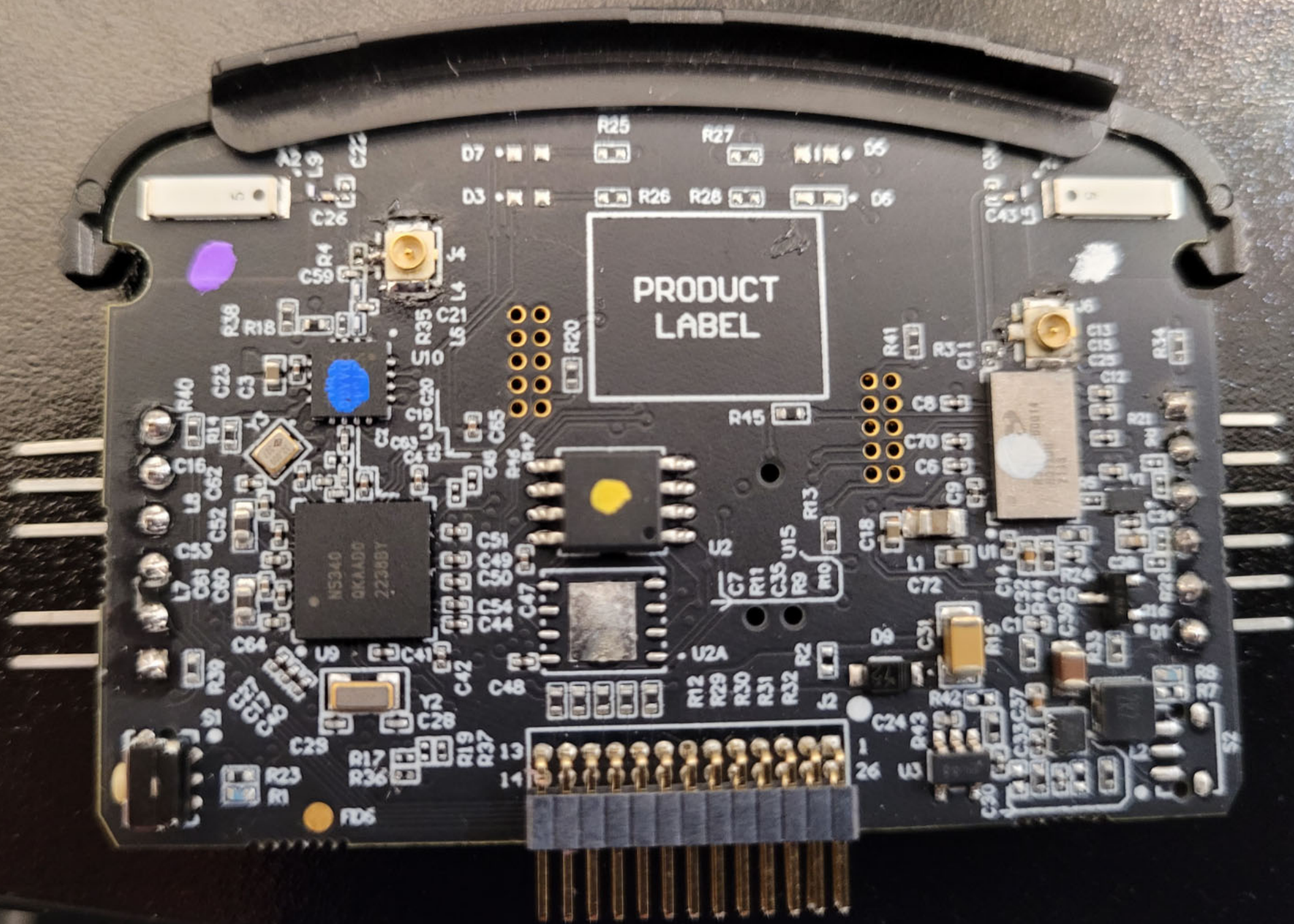
Top View of the RF Module with Label Removed - View 1
