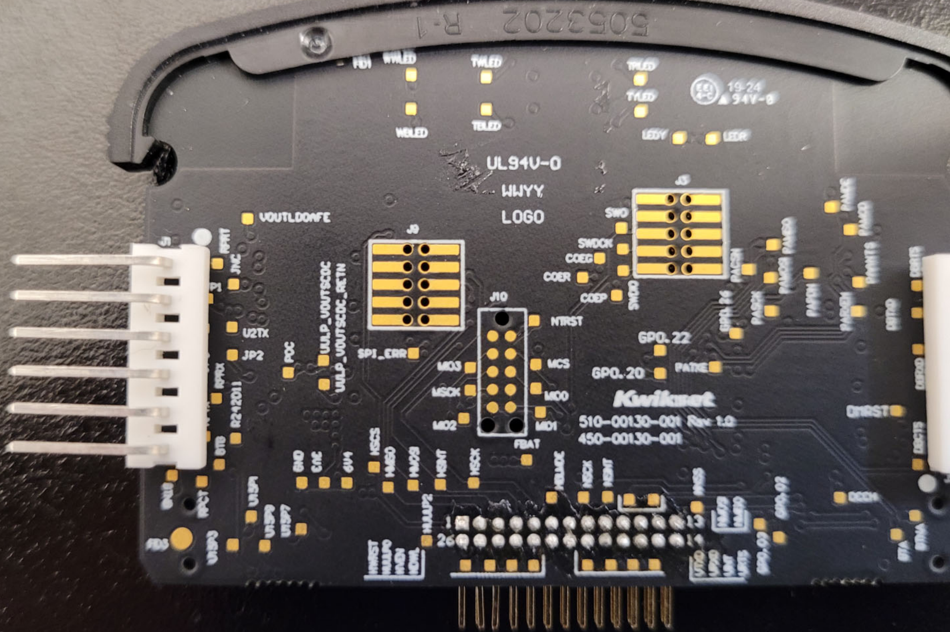
Bottom View of the RF Module with Label - View 4
