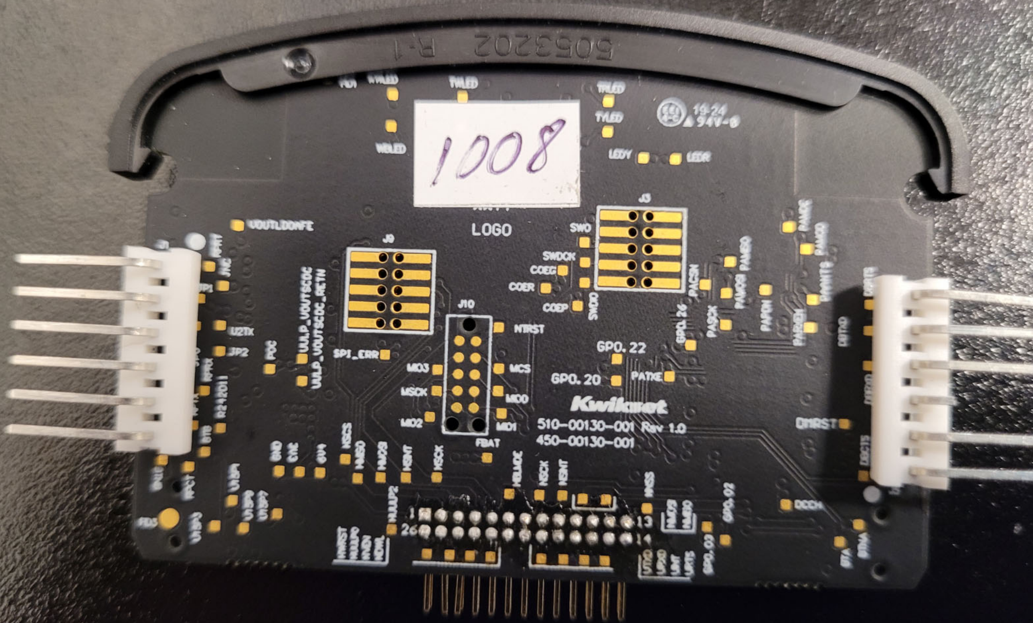
Bottom View of the RF Module with Label
