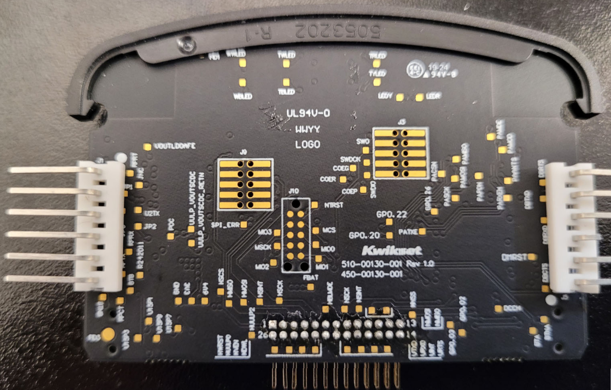
Bottom View of the RF Module with Label - View 3
