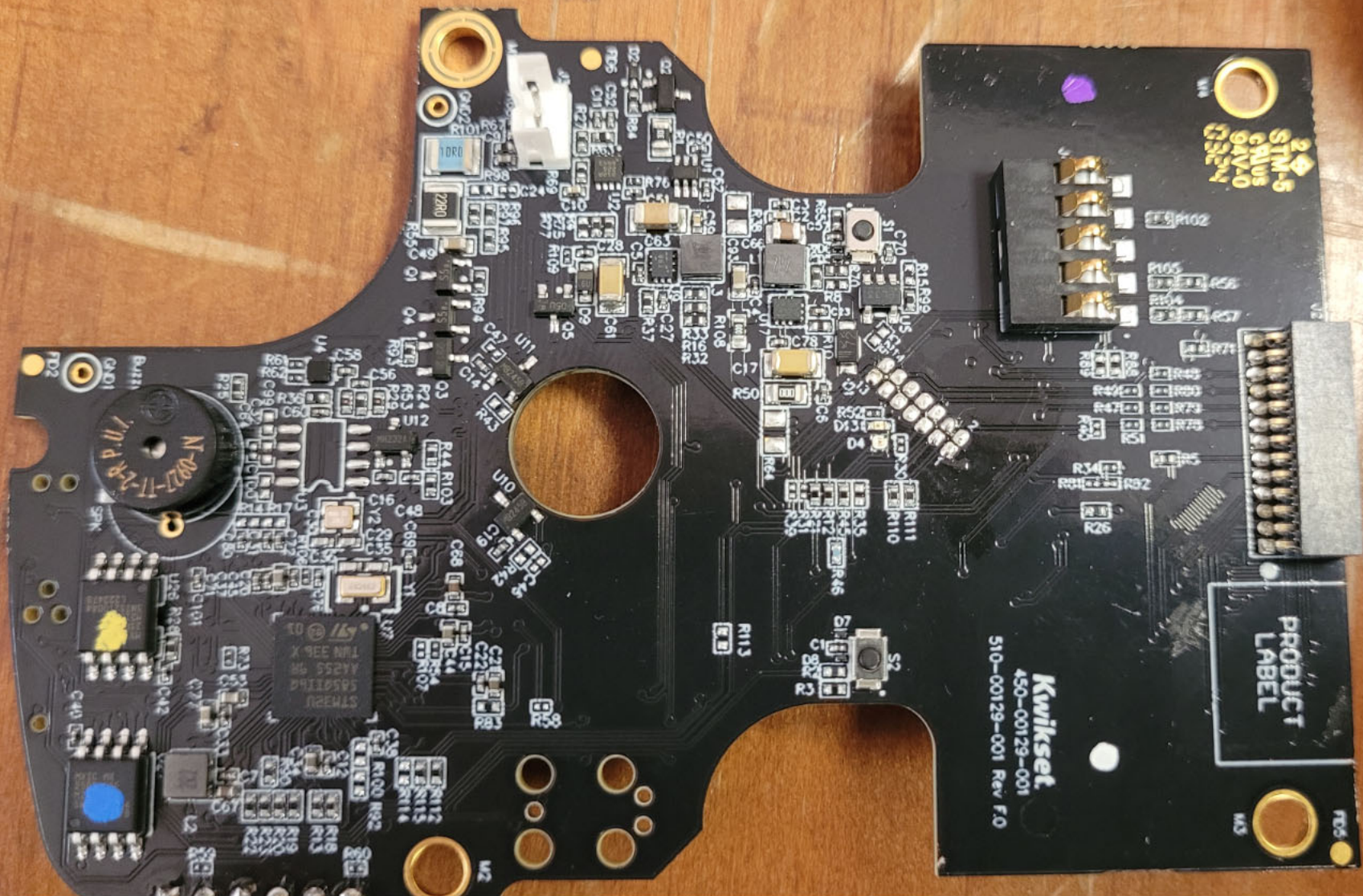
Bottom View of the PCB - #3
