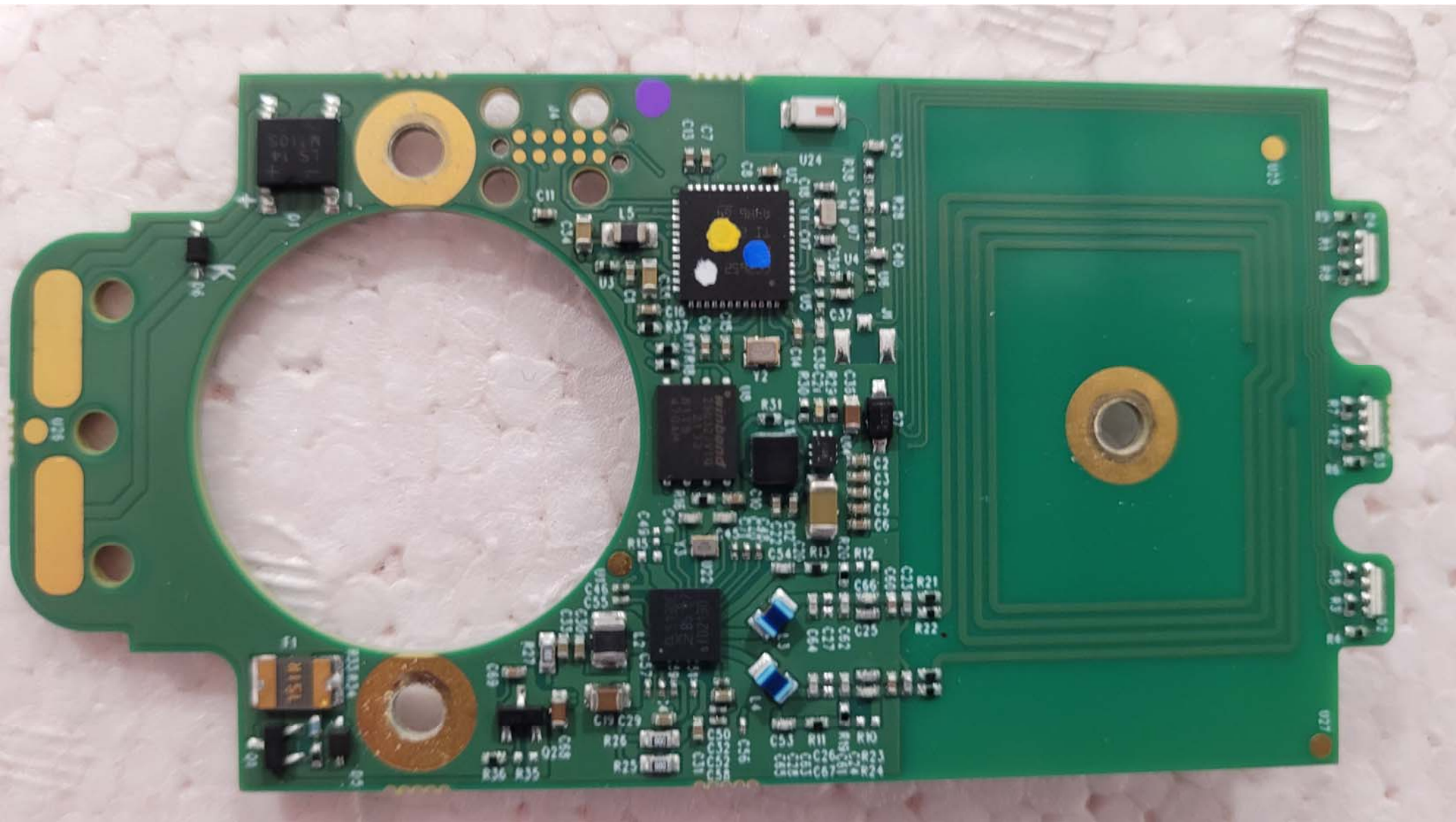
Top View of the RFID PCB for the EUT - View #2
