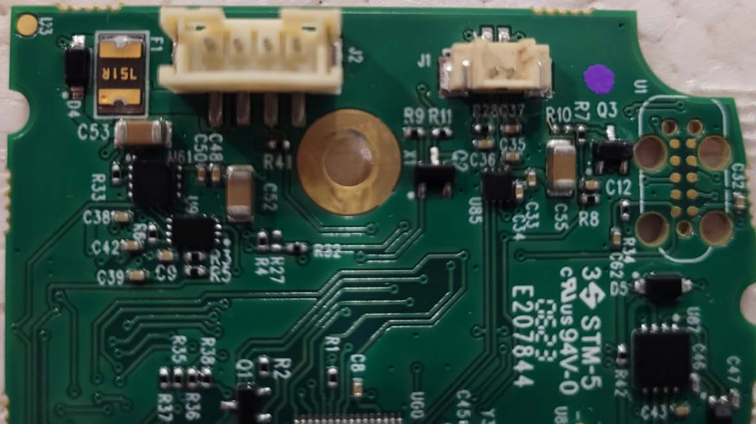
Top View of the Main PCB - Closeup #4
