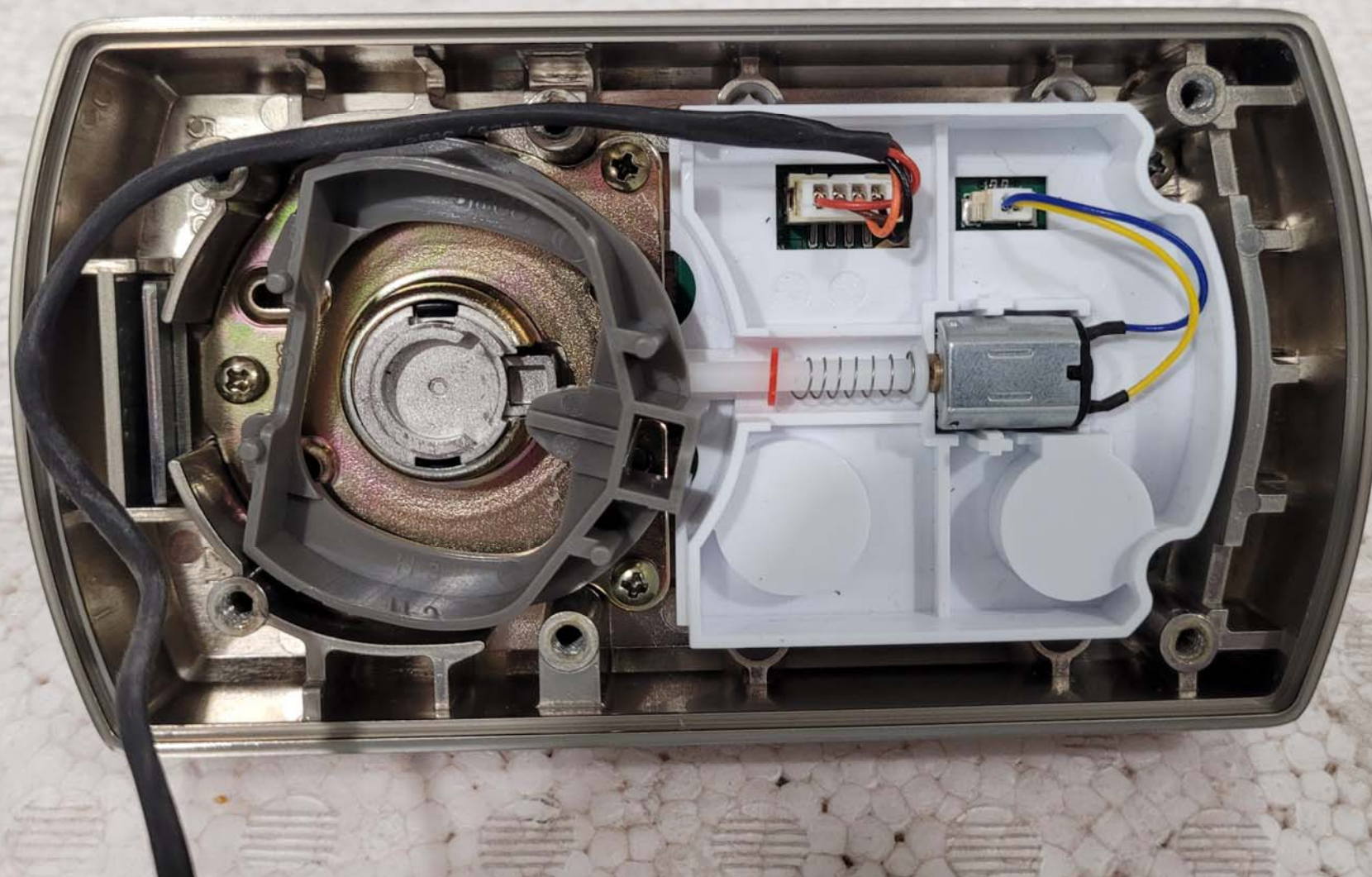
Inside View of the EUT - View #2
