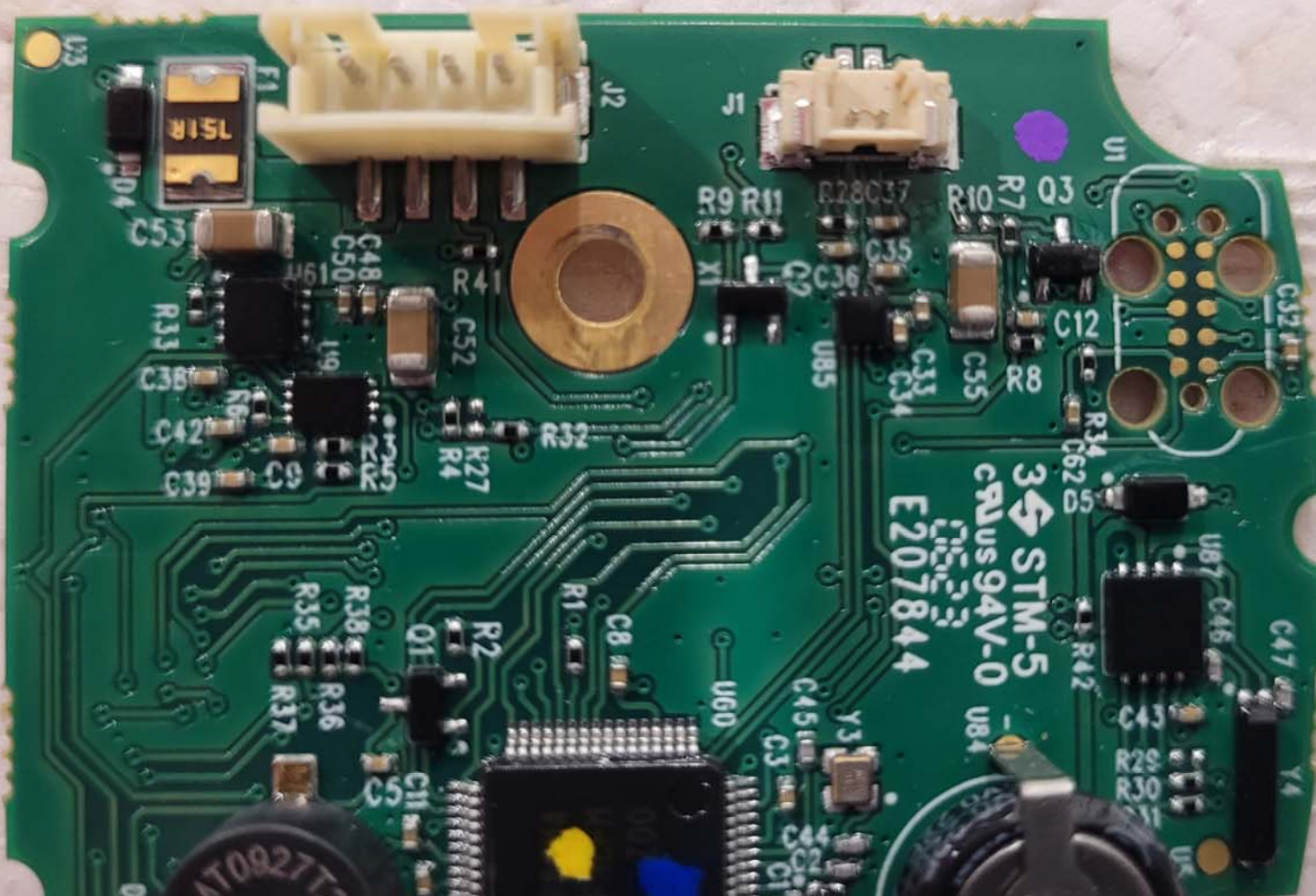
Top View of the Main PCB - Closeup #5
