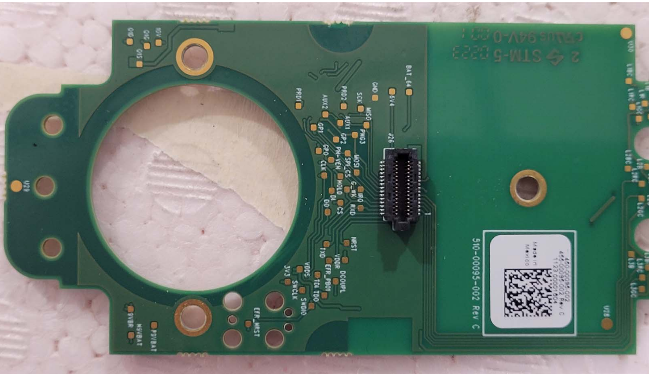
Bottom View of the RFID PCB for the EUT - View #1
