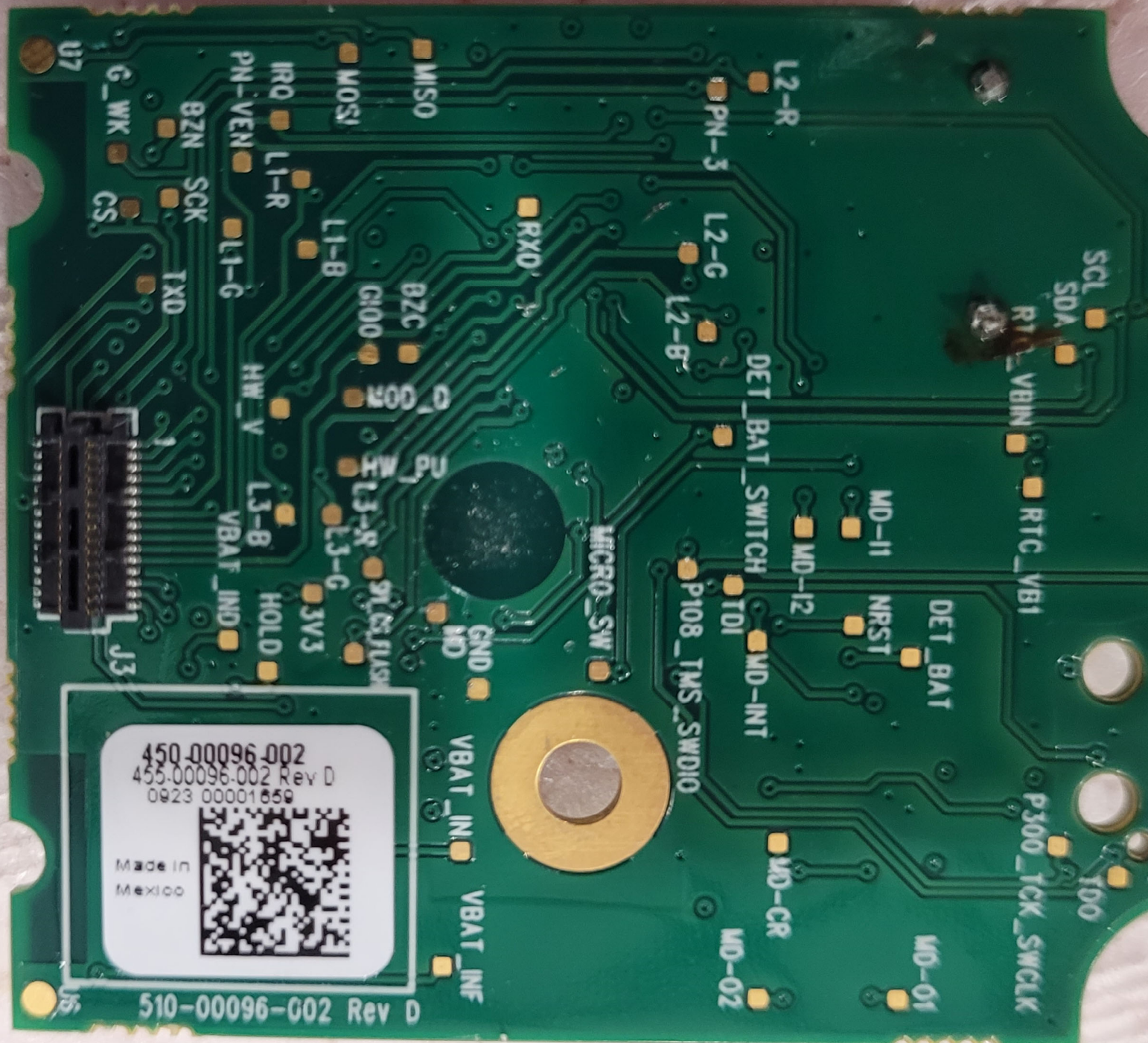
Bottom View of the Main PCB of the EUT - View #1
