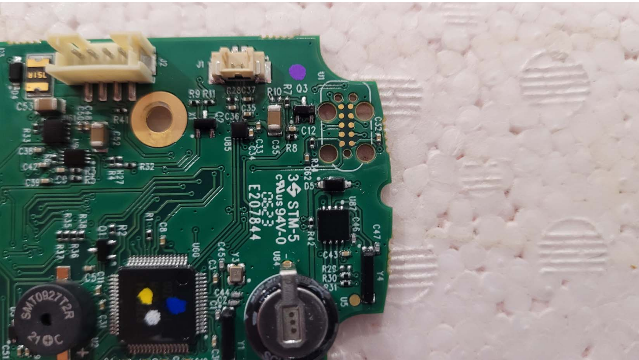
Top View of the Main PCB - Closeup #6
