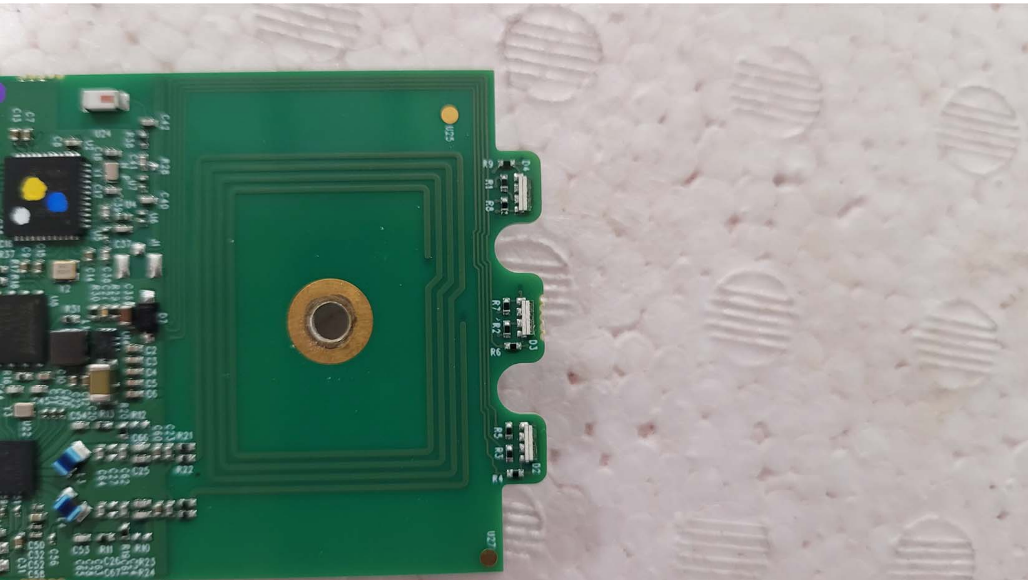
Top View of the RFID PCB for the EUT - Closeup #4
