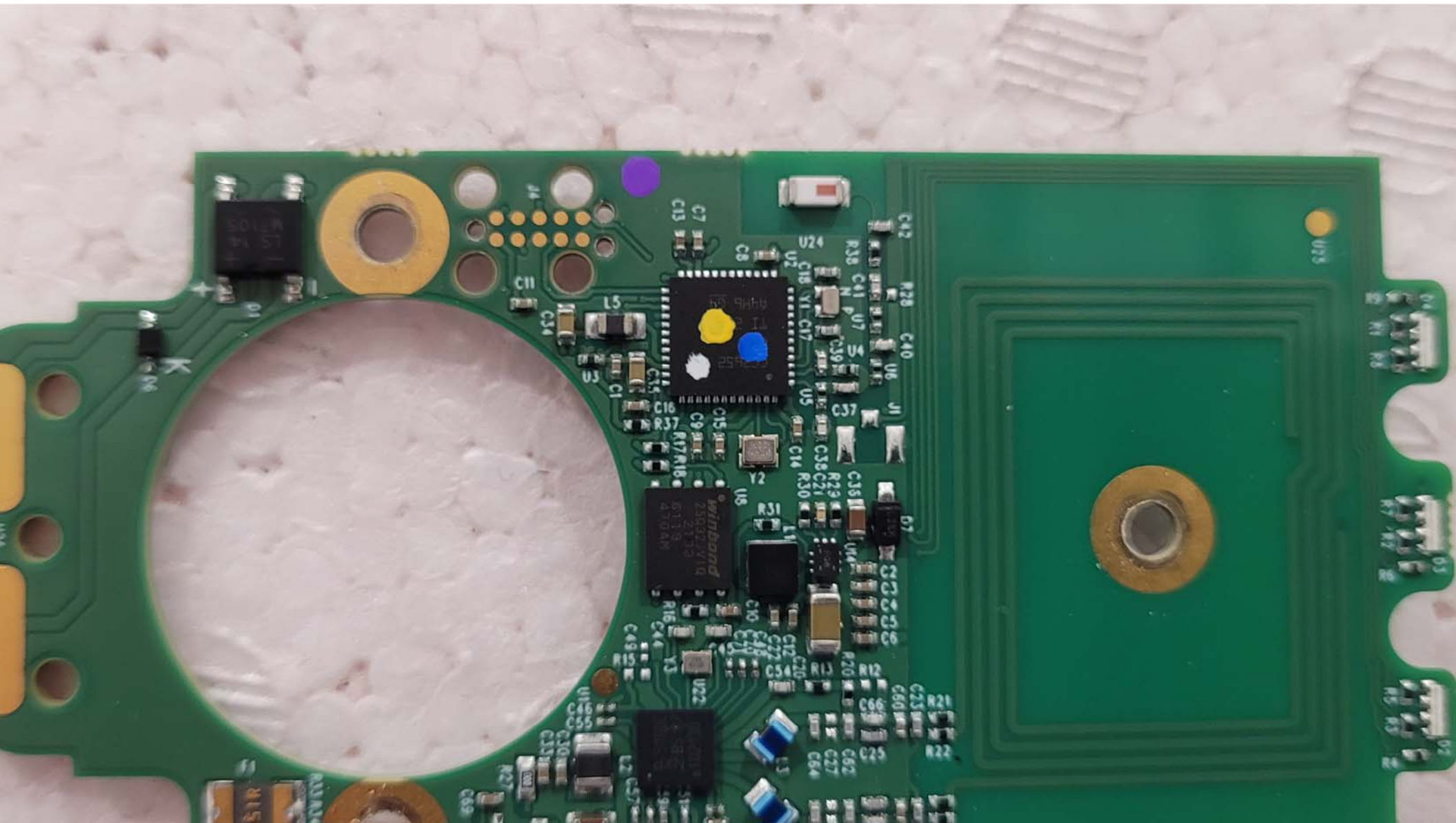
Top View of the RFID PCB for the EUT - Closeup #2
