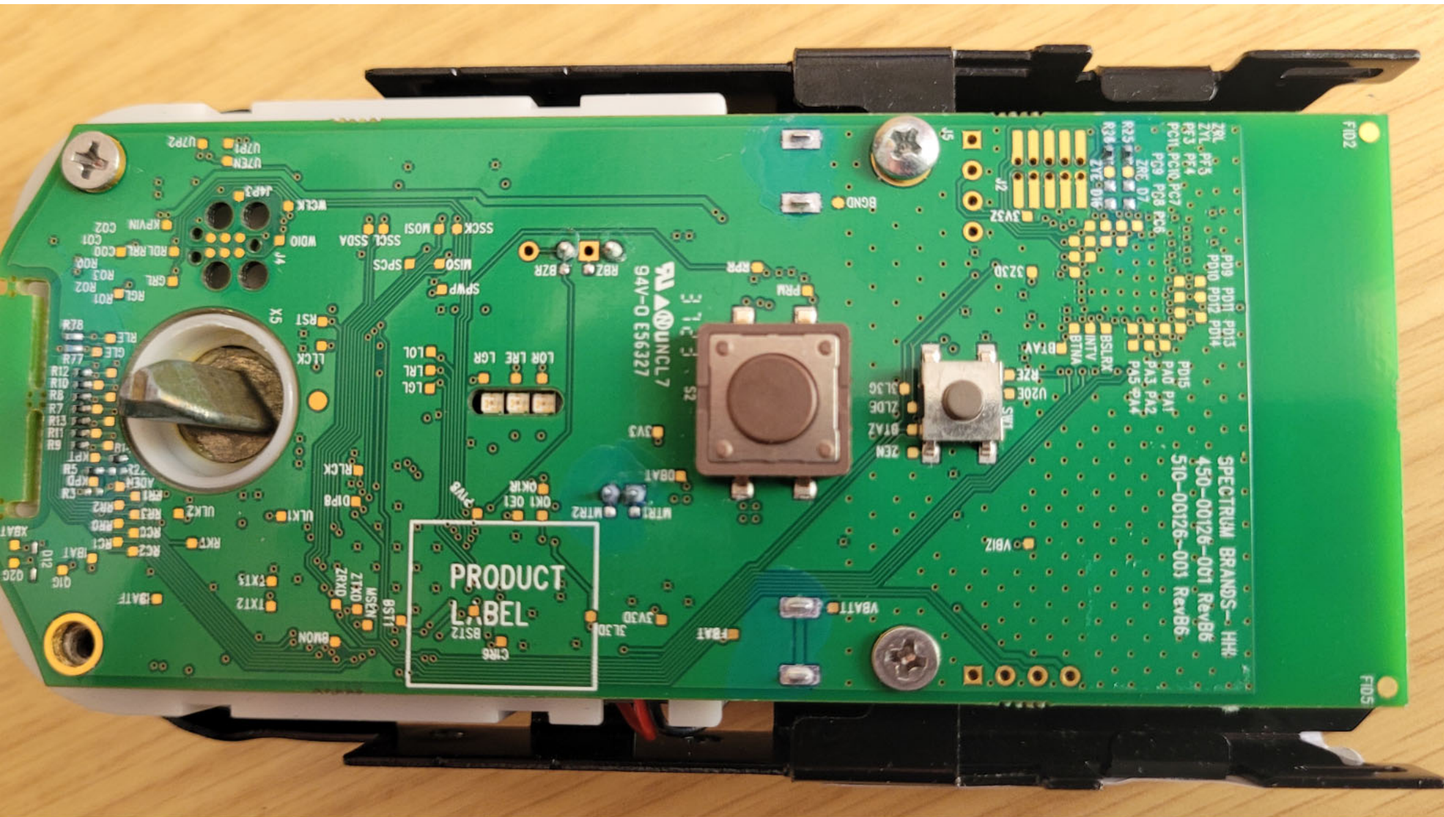
Top View of the PCB - View #1 - HVIN: GED1800
