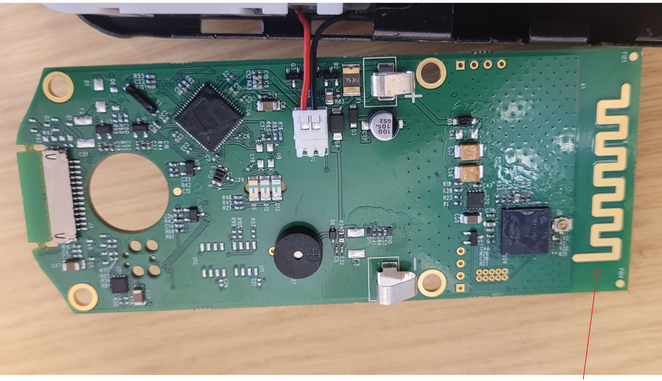
Bottom View of the PCB - View #1 - HVIN: GED1800
