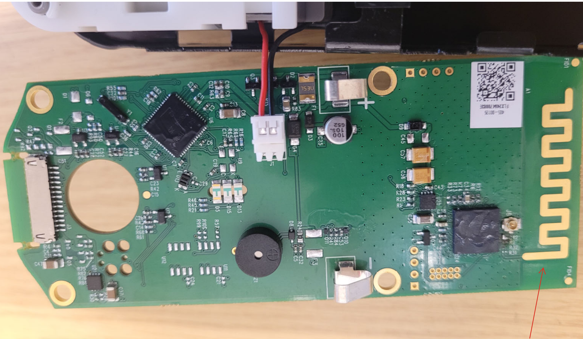
Bottom View of the PCB - View #3 - HVIN: GED1800
