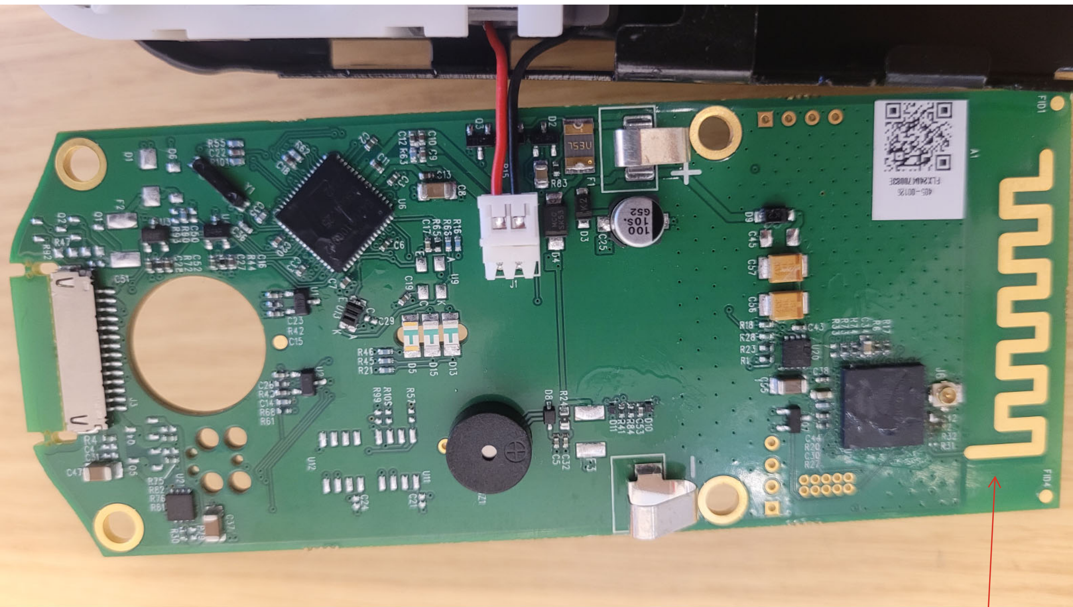
Bottom View of the PCB - View #4 - HVIN: GED1800
