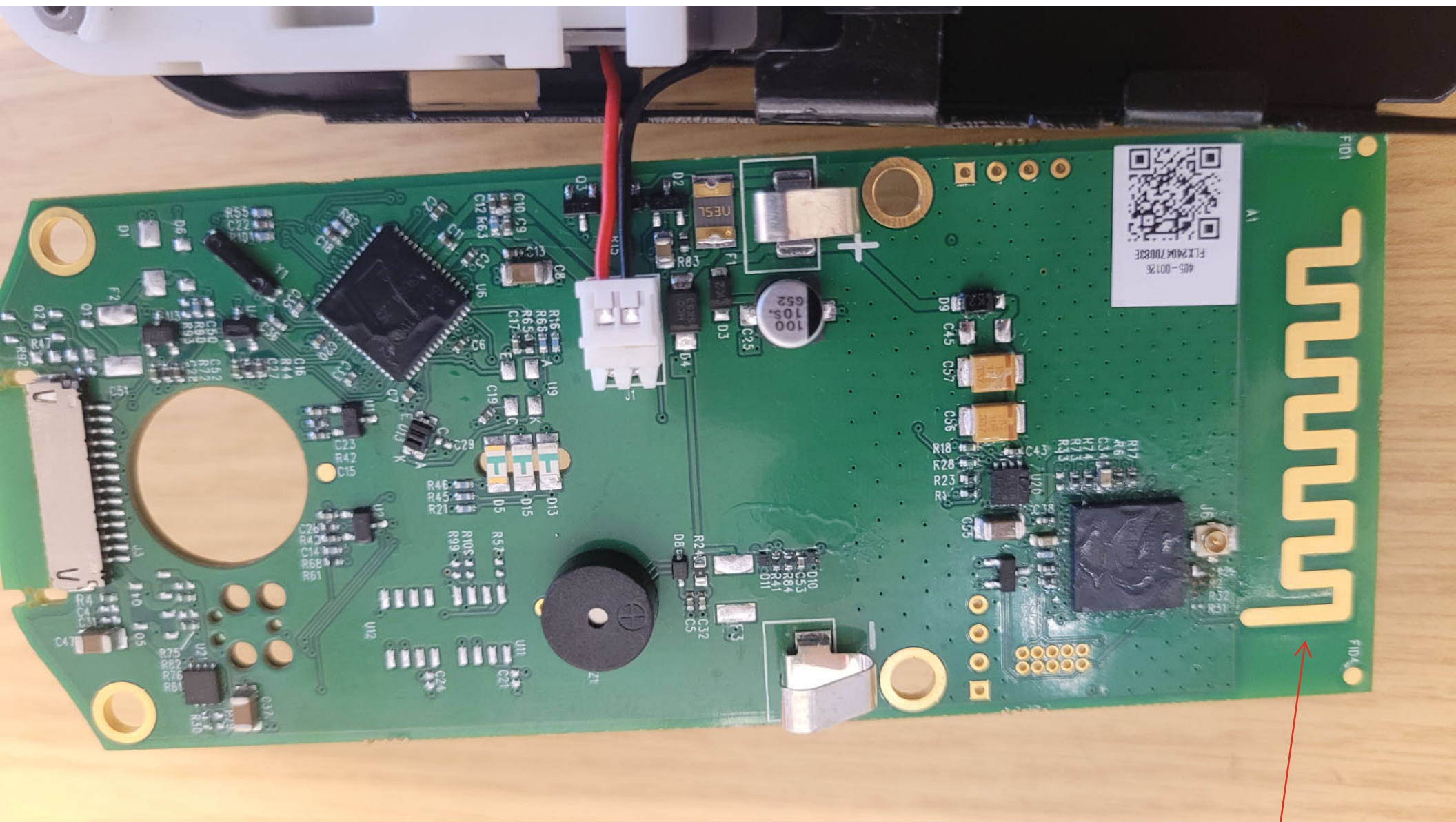
Bottom View of the PCB - View #2 - HVIN: GED1800
