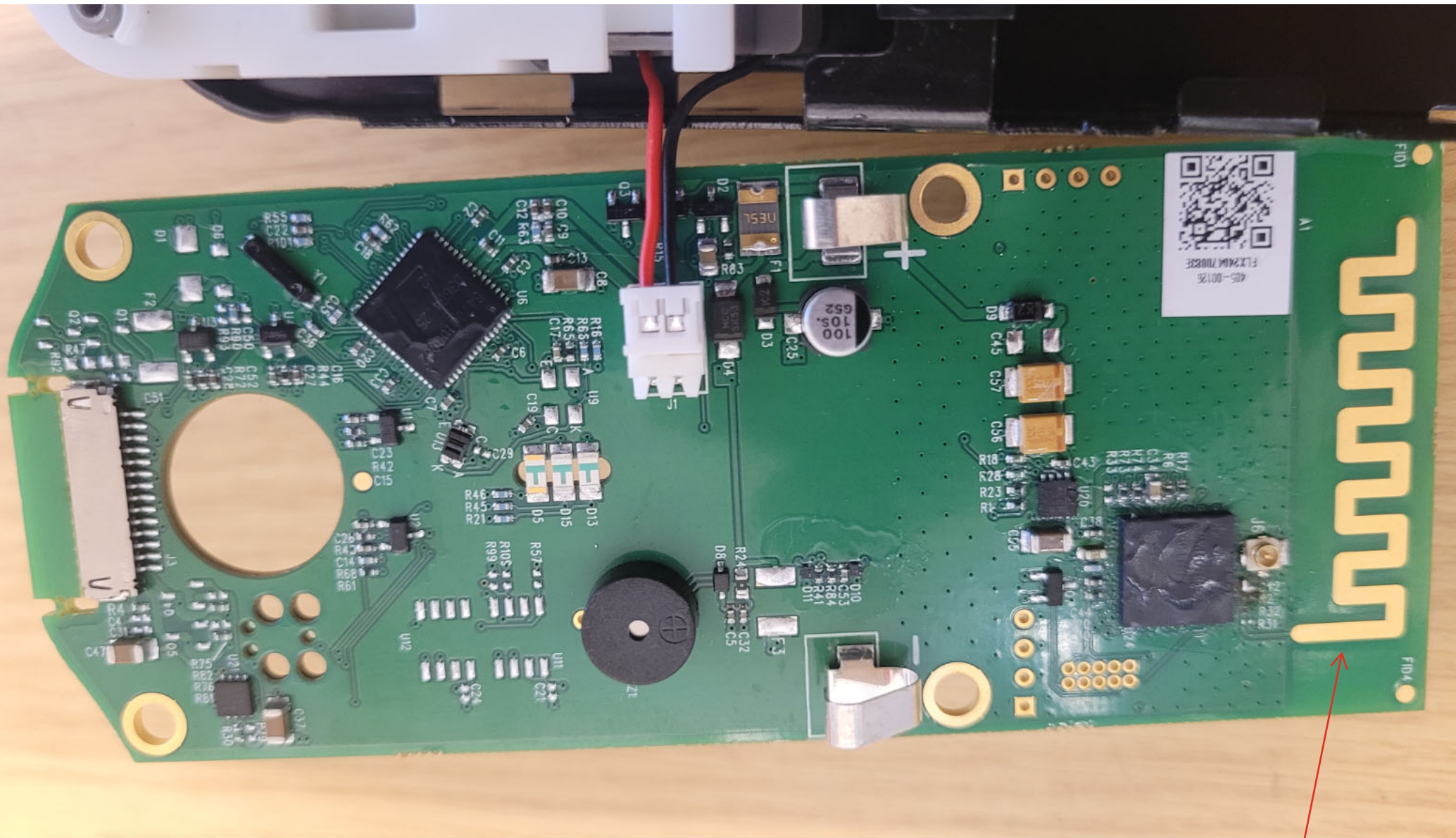
Bottom View of the PCB - View #3 - HVIN: GED2152
