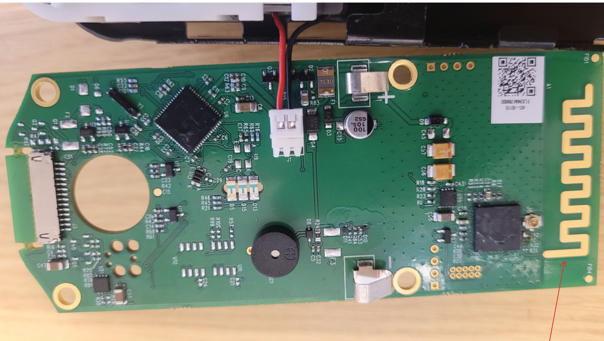
Bottom View of the PCB - View #4 - HVIN: GED2152
