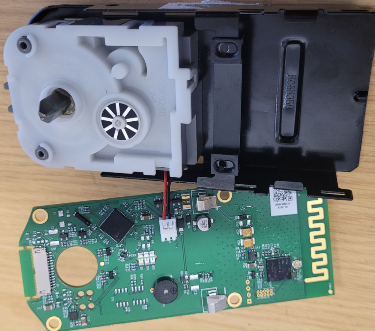
Inside View of the EUT - #4 - HVIN: GED2152
