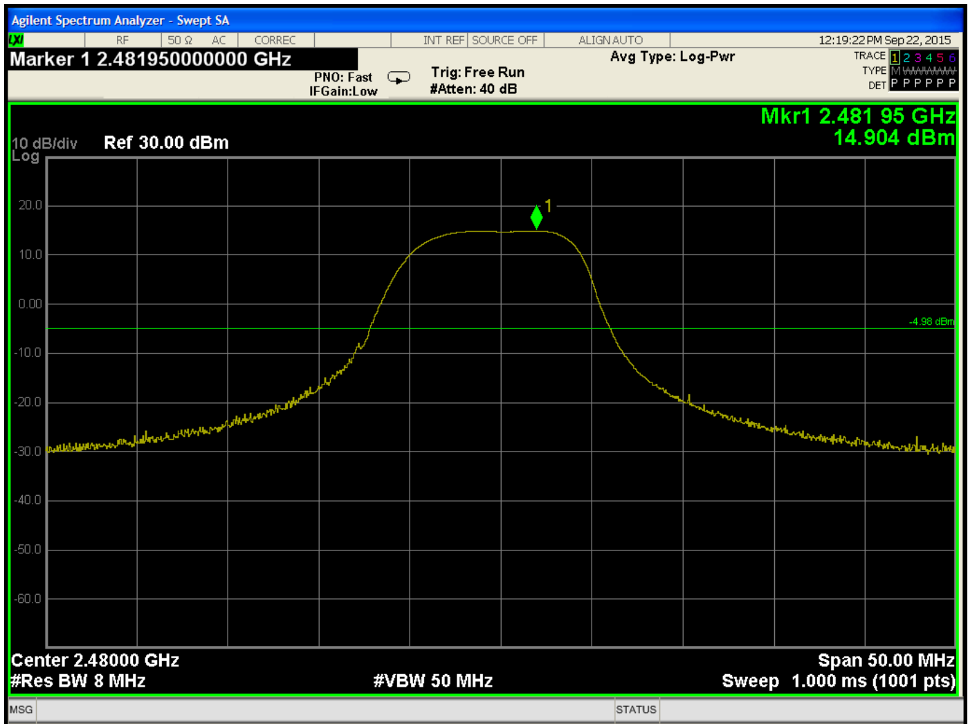
Peak Power Output – 2480 MHz
