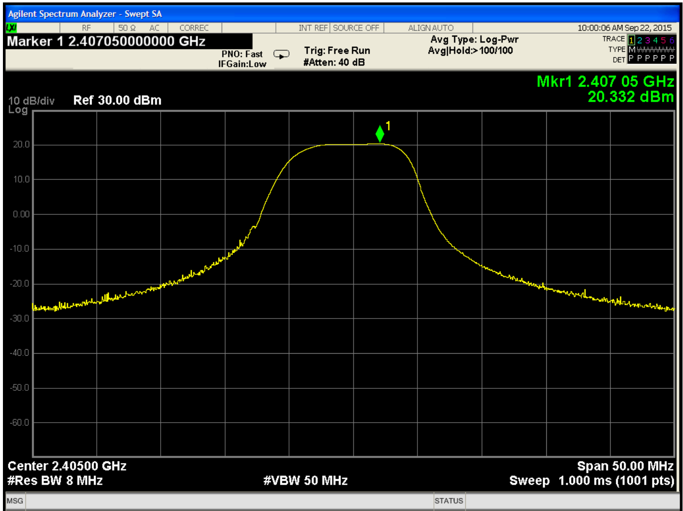
Peak Power Output – 2405 MHz
