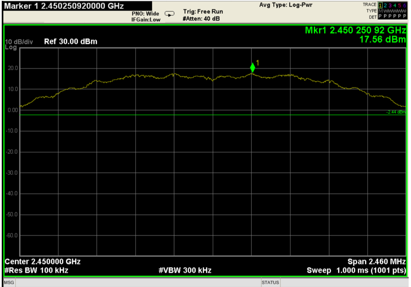
RF Antenna Conducted – Reference Level – 2450 MHz Fundamental
