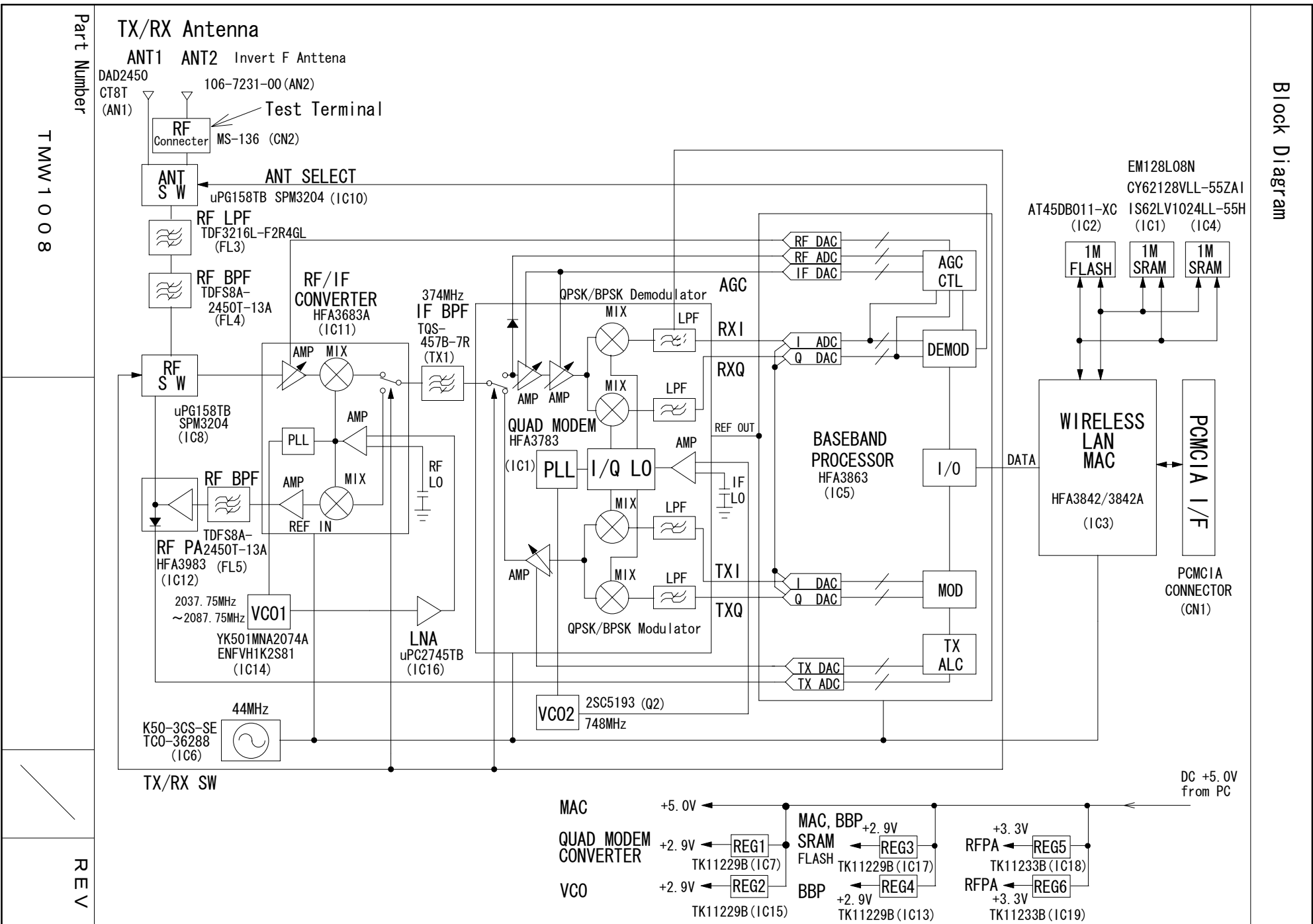
ANNEX C Figure 4.1 Block Diagram of FCC ID: NUSTMW1008
