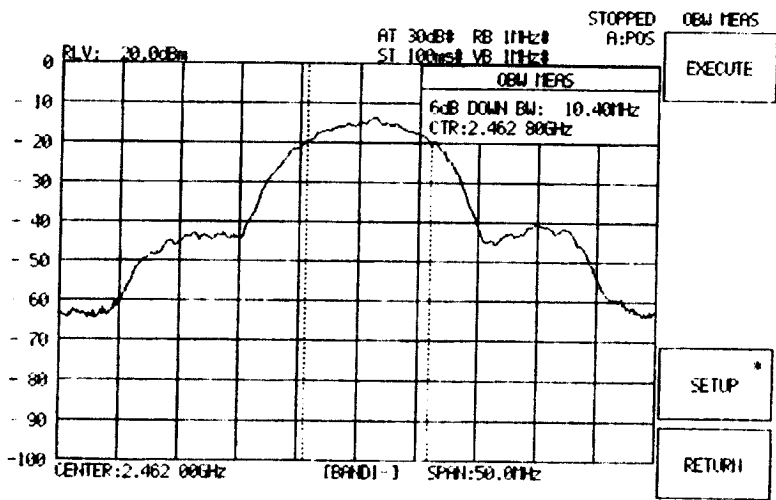
Fig CH11 (2462MHz)
