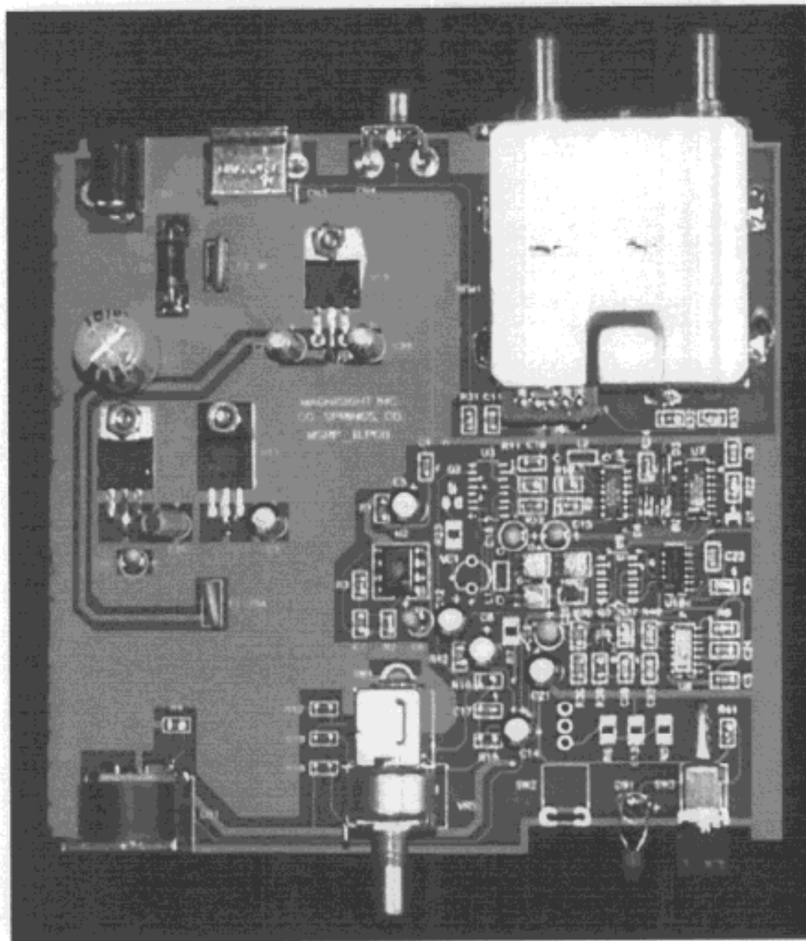
FCC ID: NUUMCB05 Photo 4 Main Board, Component Side
