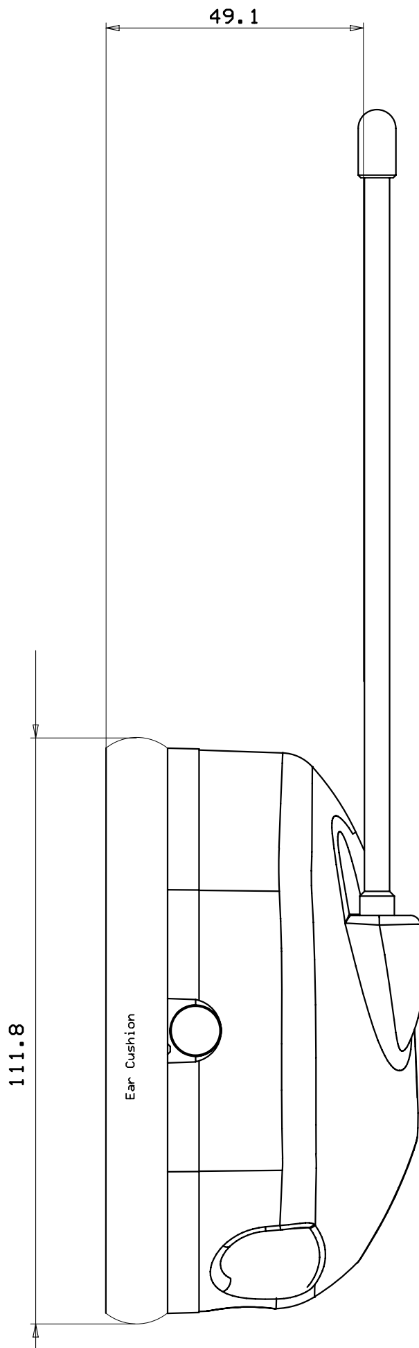
P522/526 Head to Antenna distance (mm) Peltor 040218
