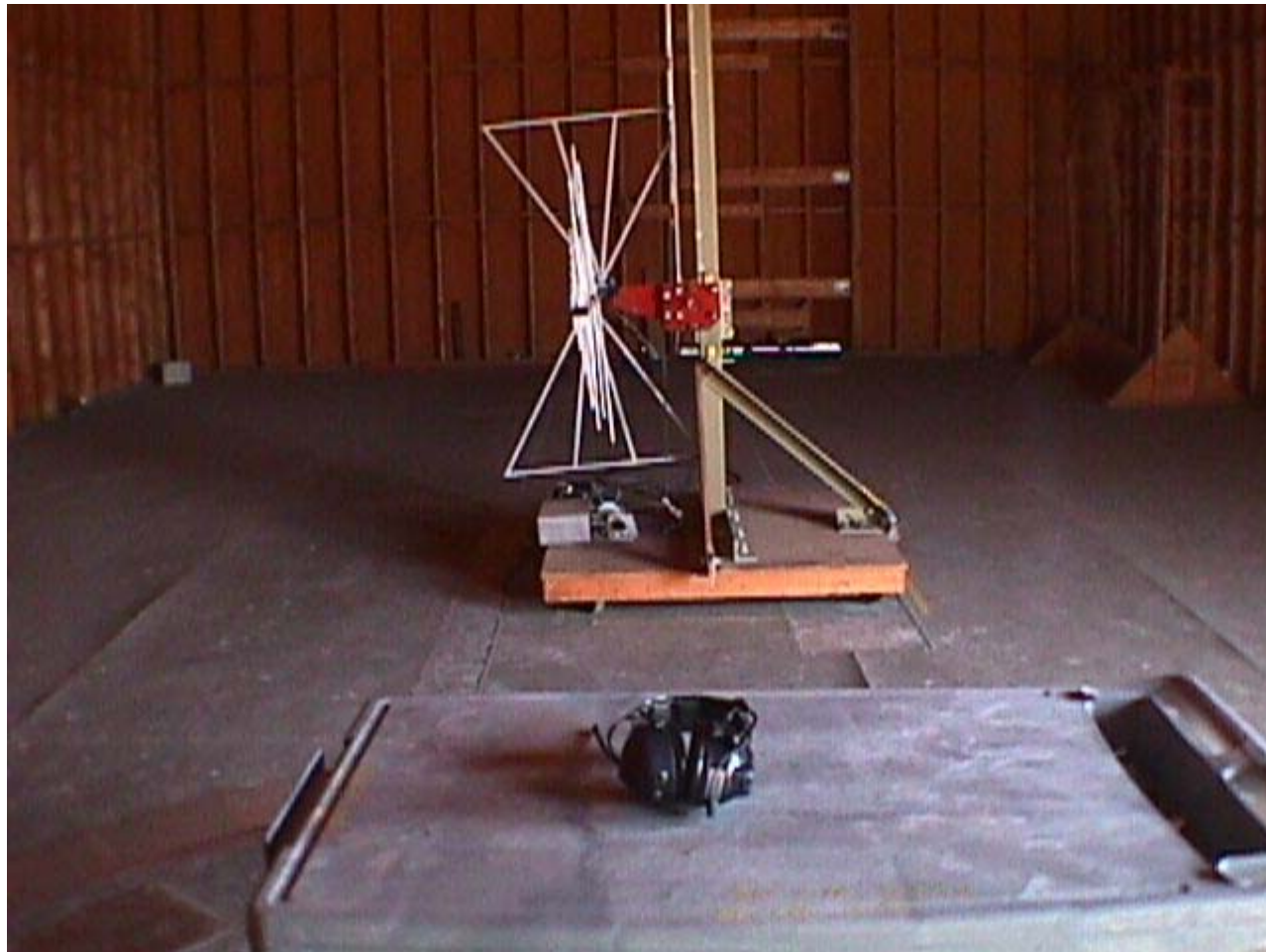
Radiated Emissions at 3 Meters Distance Orthogonal Position # 1
