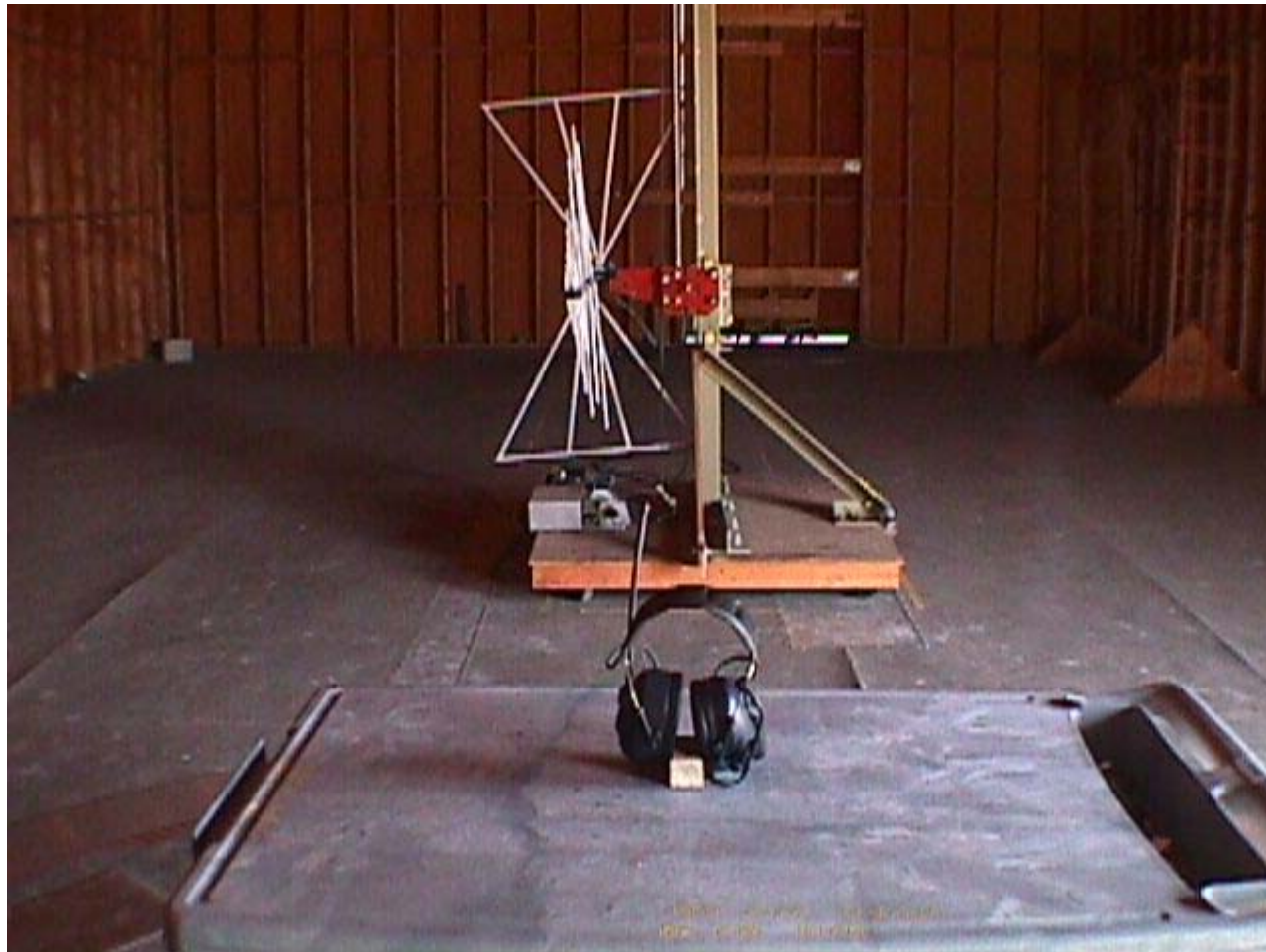
Radiated Emissions at 3 Meters Distance Orthogonal Position # 3
