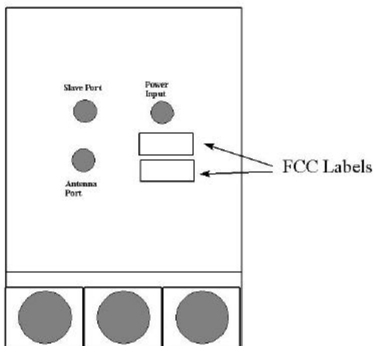
REMOTE UNIT, LABEL LOCATIONS (REAR VIEW)
