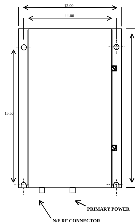
OUTLINE DRAWING
