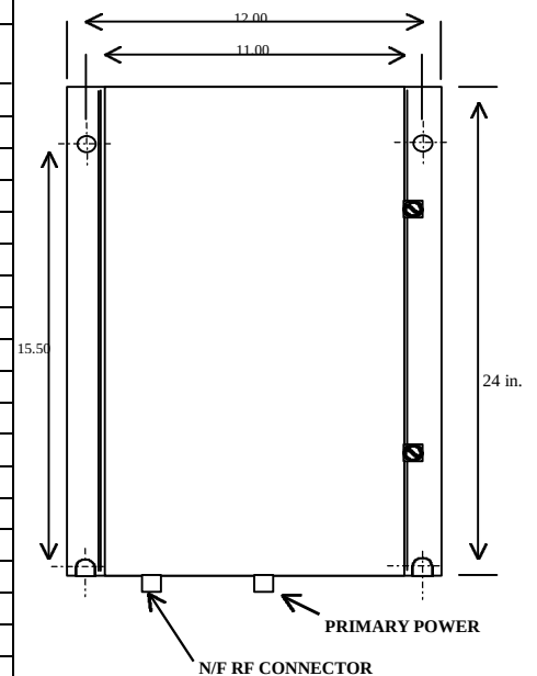
OUTLINE DRAWING
