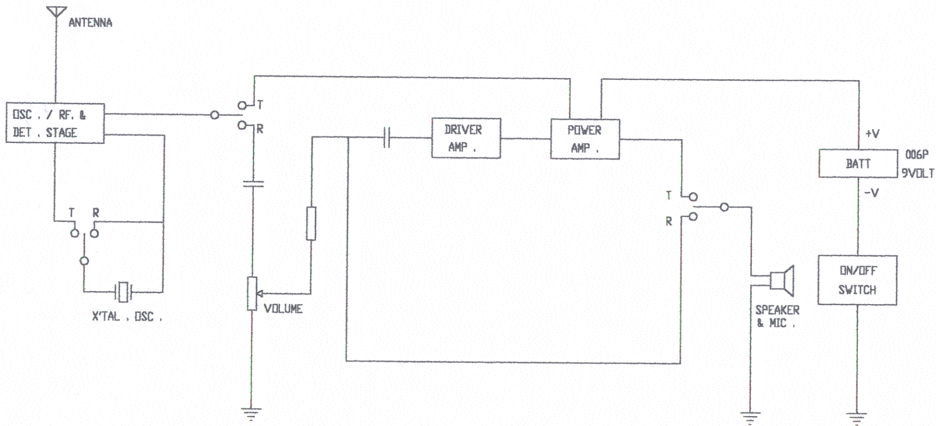
BLOCK DIAGRAM
