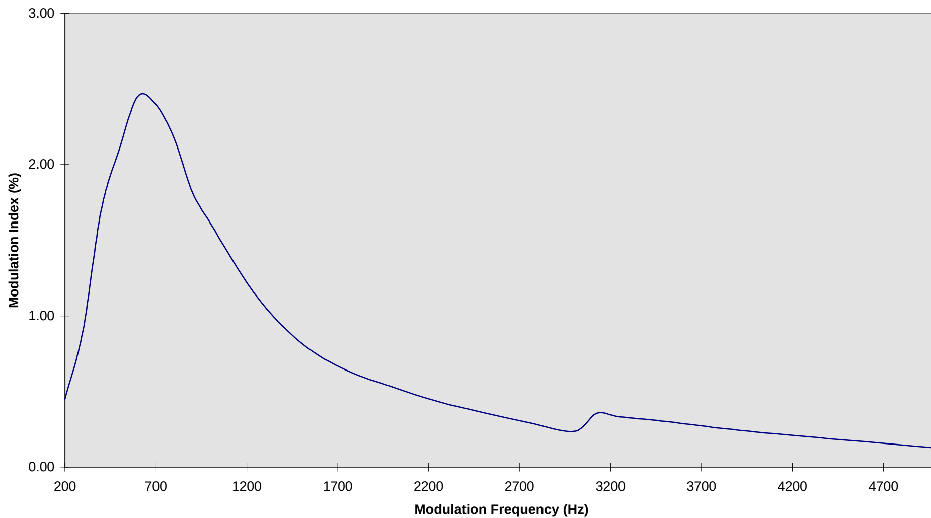
Modulation Frequency Response (Model: UBZ-AR14)
