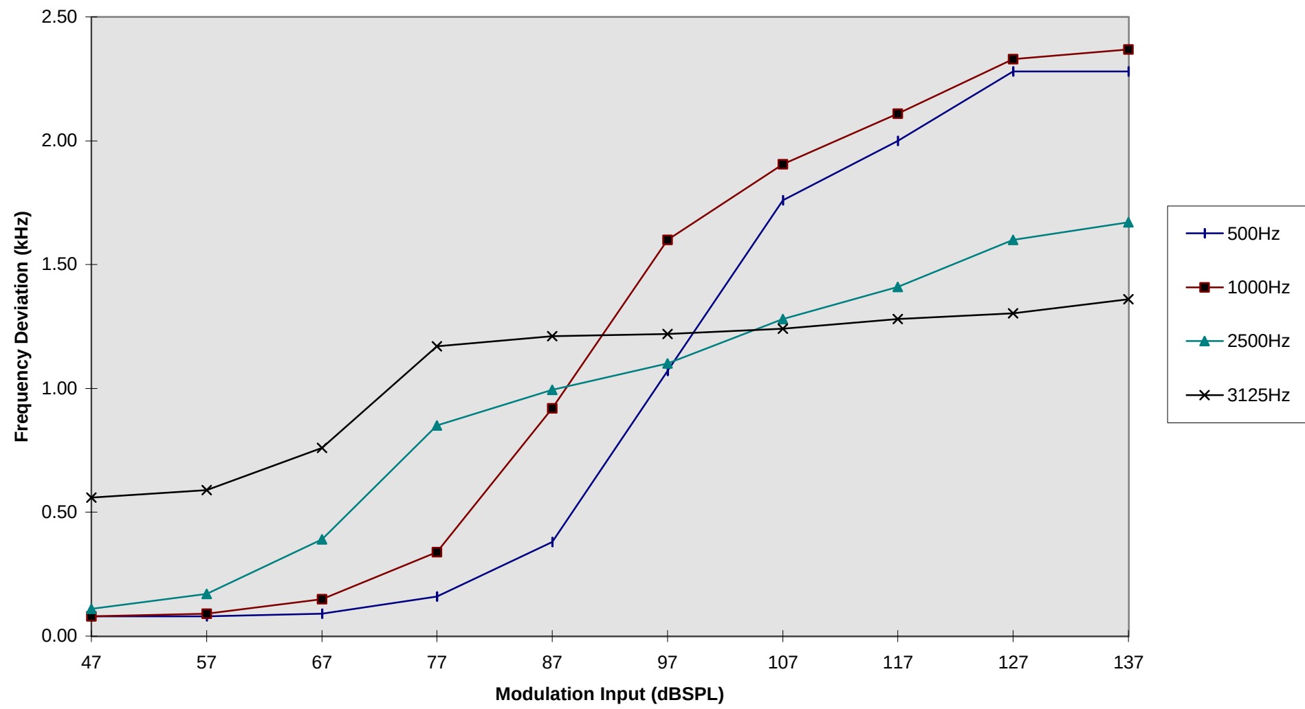
Modulation Limiting Characteristic (Model: UBZ-AR14)
