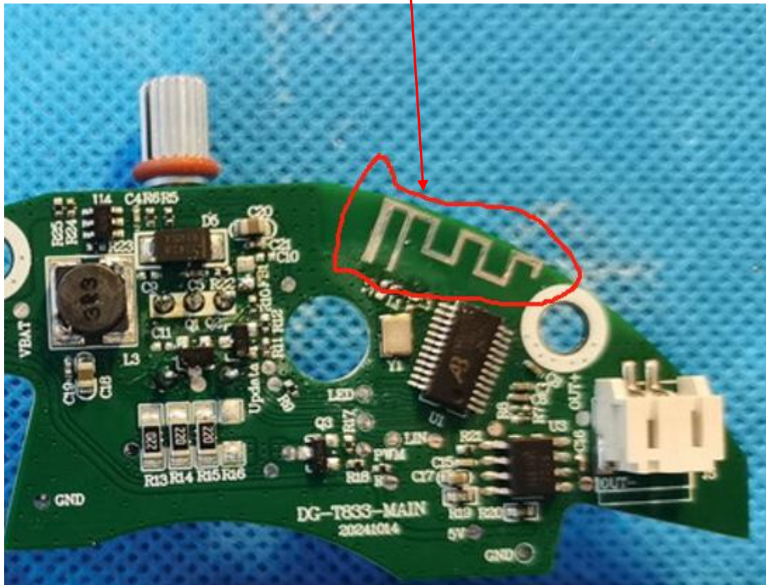
BT antenna
