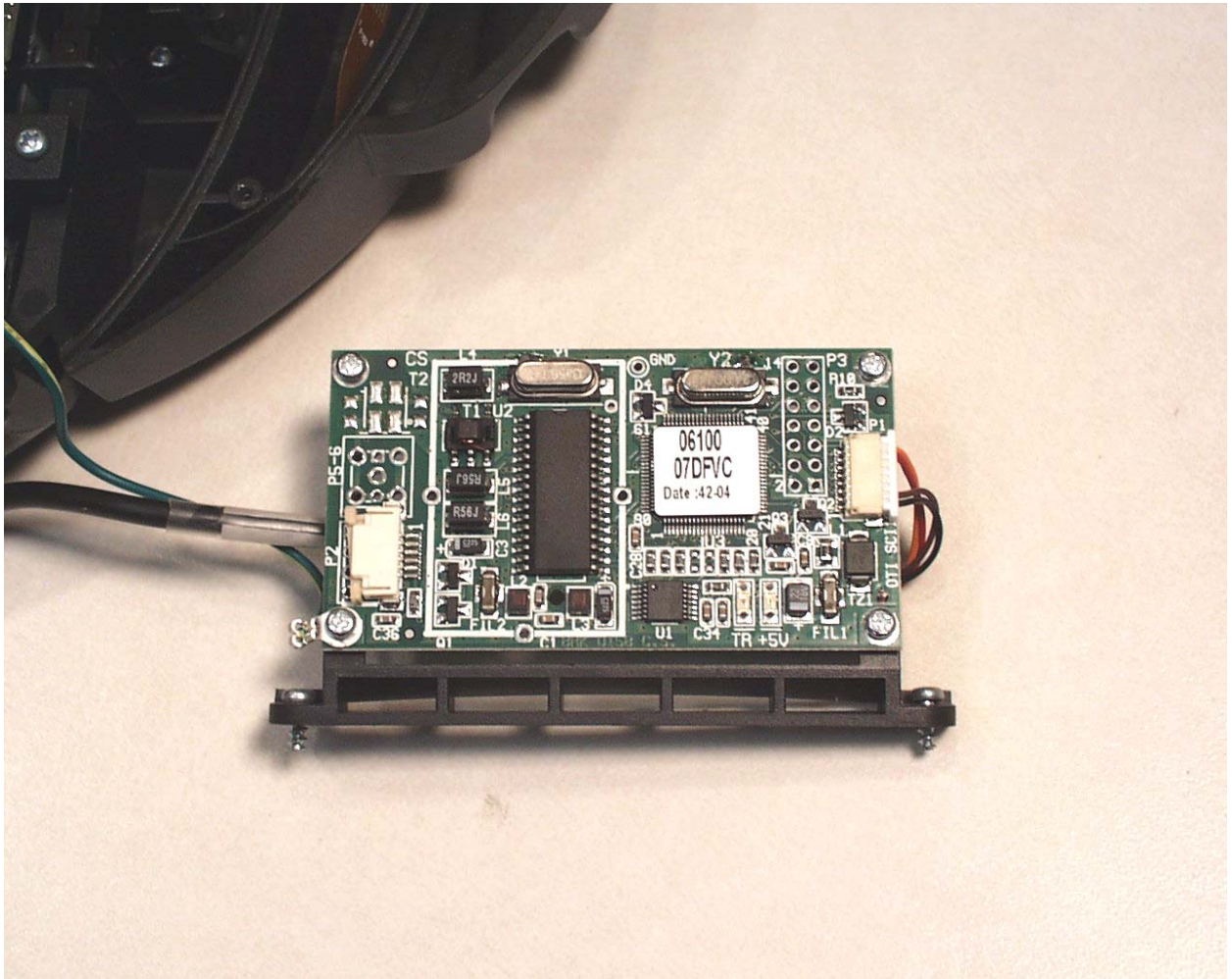
View of the Magnetic Card Reader PCB
