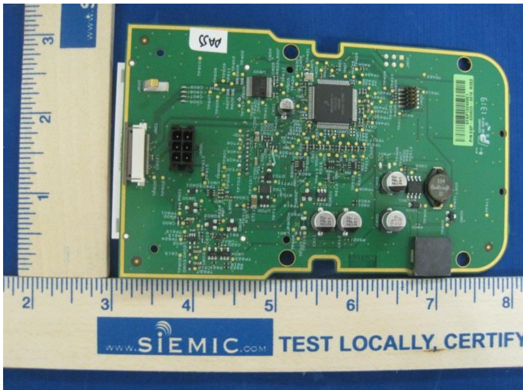
Keypad Board-Bottom View
