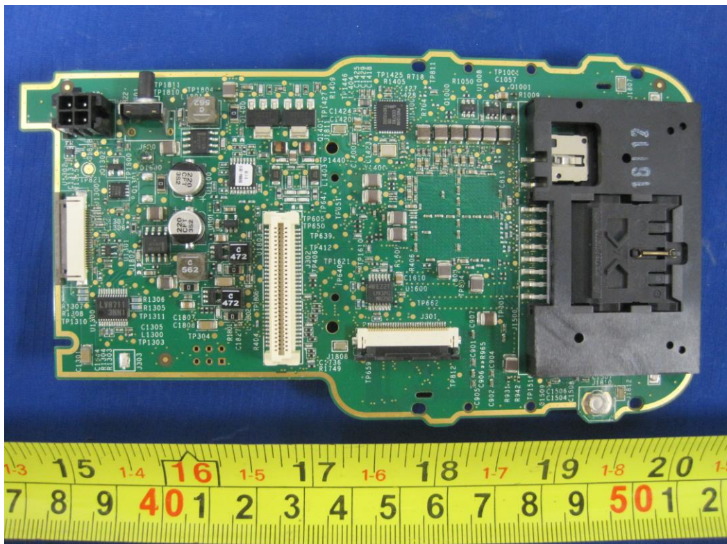
PCB 2-Bottom View
