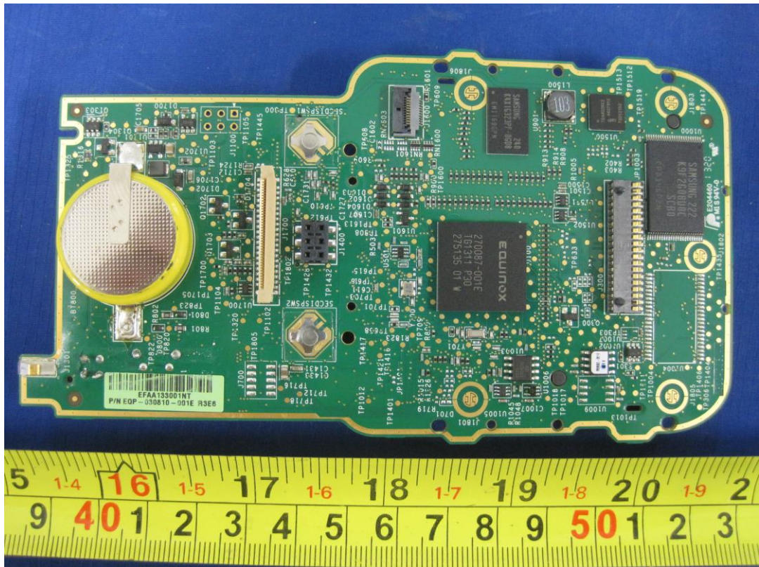
PCB 2-Top View
