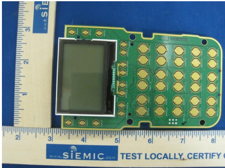
Keypad Board-Top View
