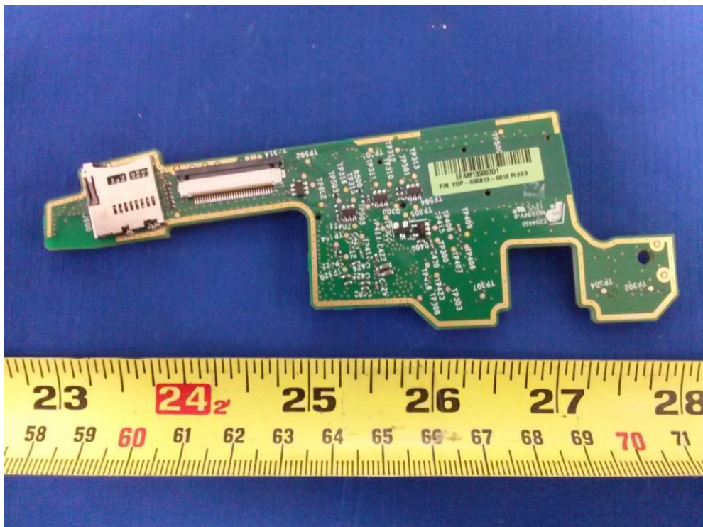
Radio Module-Bottom View
