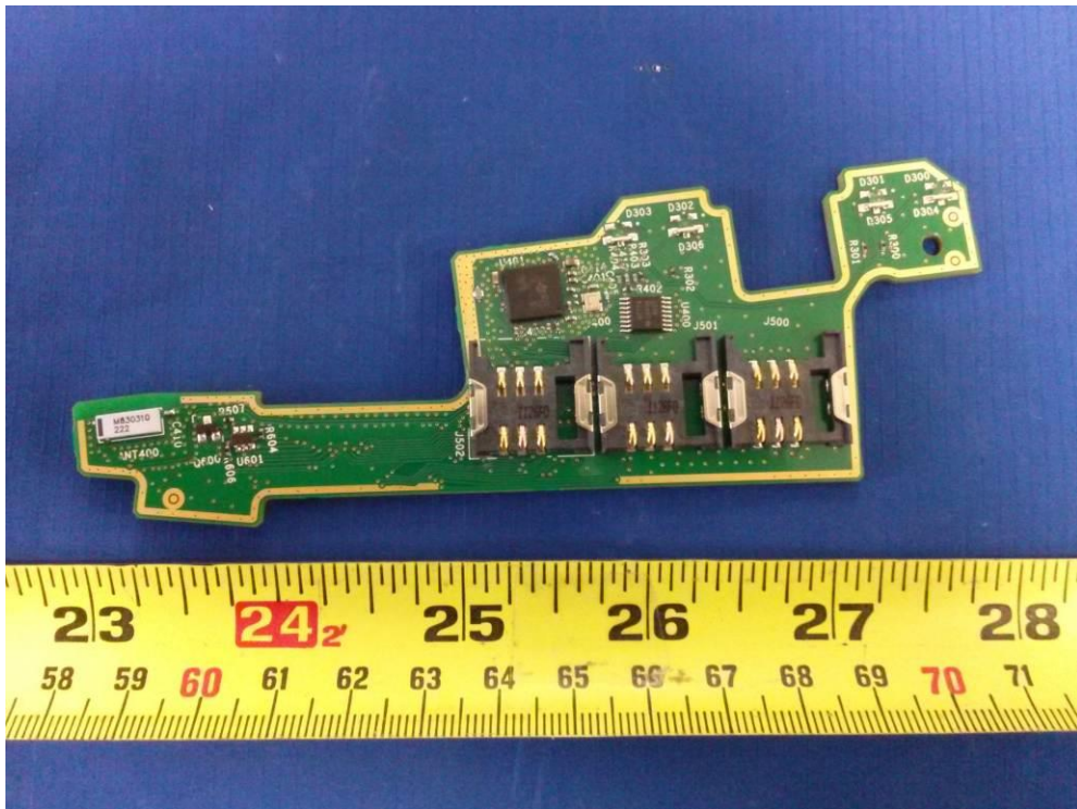
Radio Module-Top View
