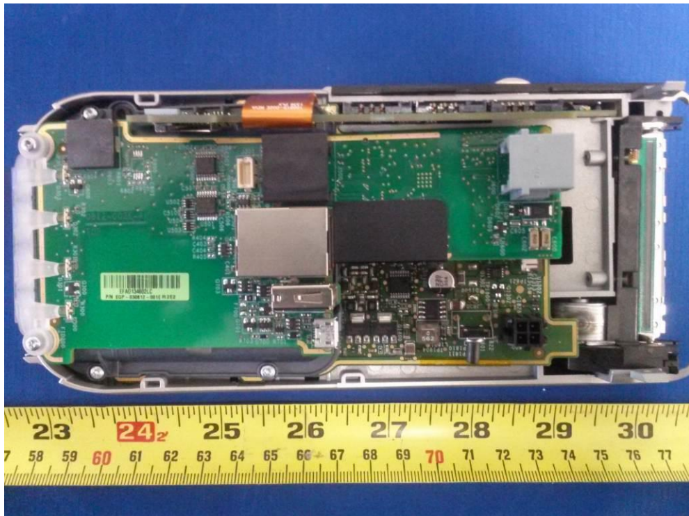
EUT Main Board
