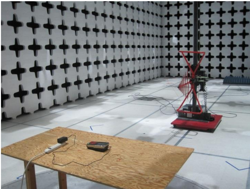
Radiated Emission (<1GHz) – Rear View
