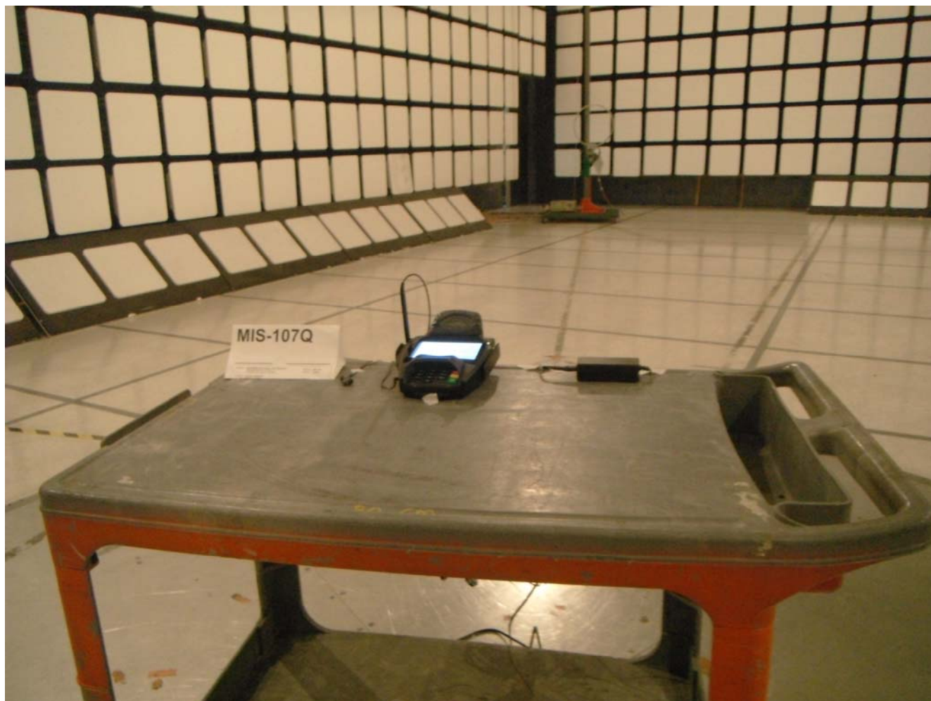
Radiated Emissions @ 10 m, Below 30 MHz
