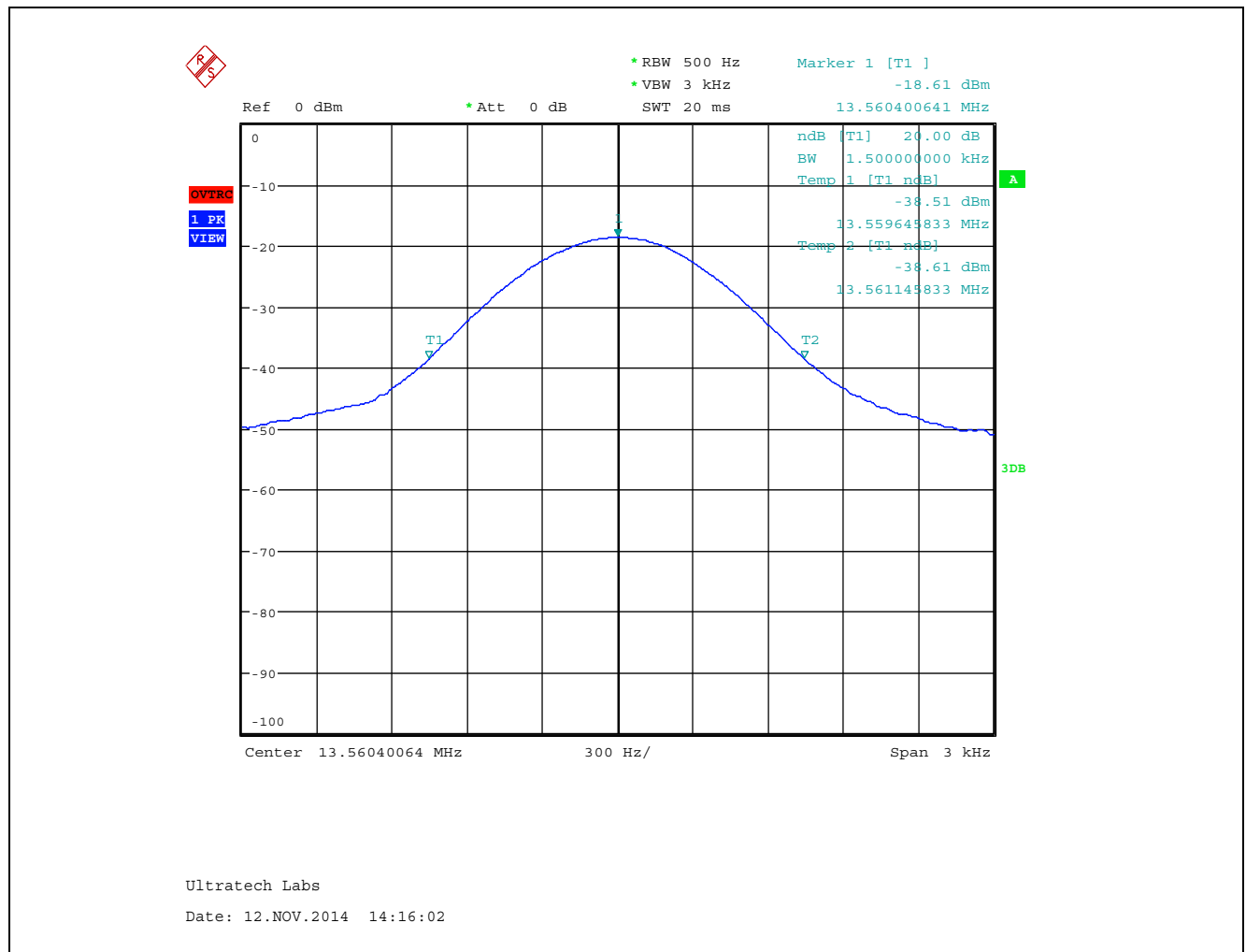
Plot 5.1.3.2. 20 dB Emission Bandwidth, 13.56 MHz
