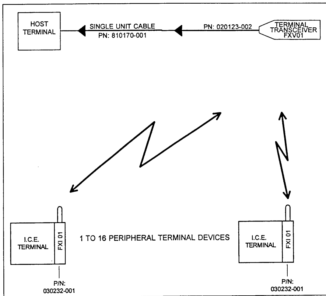
Figure 4-1. Basic configuration
