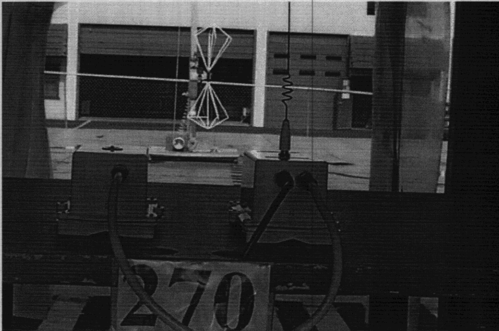
FCC Part 15.209 Radiated Emissions
