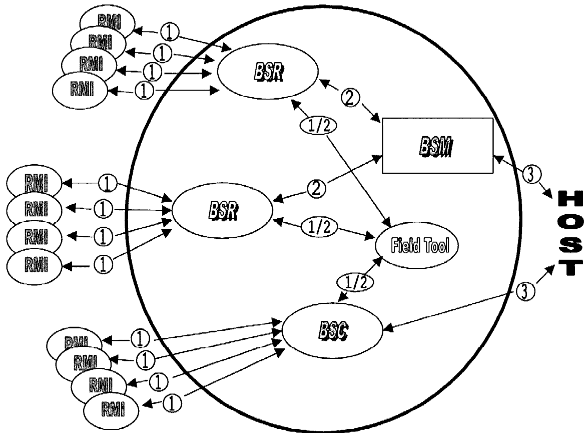
FIGURE 1 WHISPER SYSTEM ARCHITECTURE
