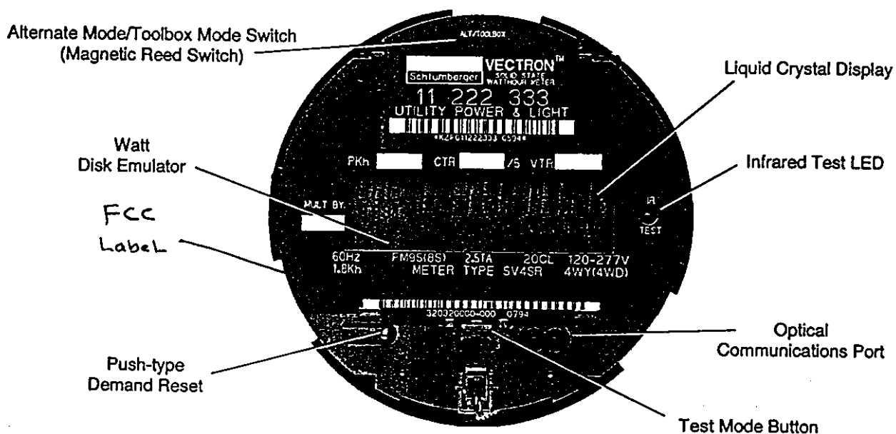
Figure 3.1 Controls and Indicators
