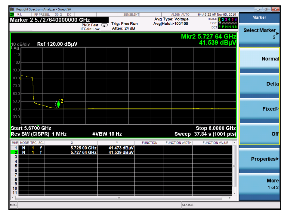
(Channel 142, AVG, 802.11n (HT40))
