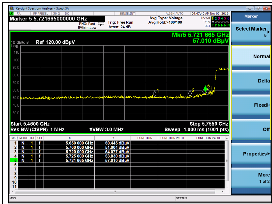
(Channel 151, PEAK, 802.11n (HT40))
