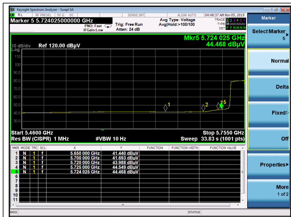
(Channel 151, AVG, 802.11n (HT40))
