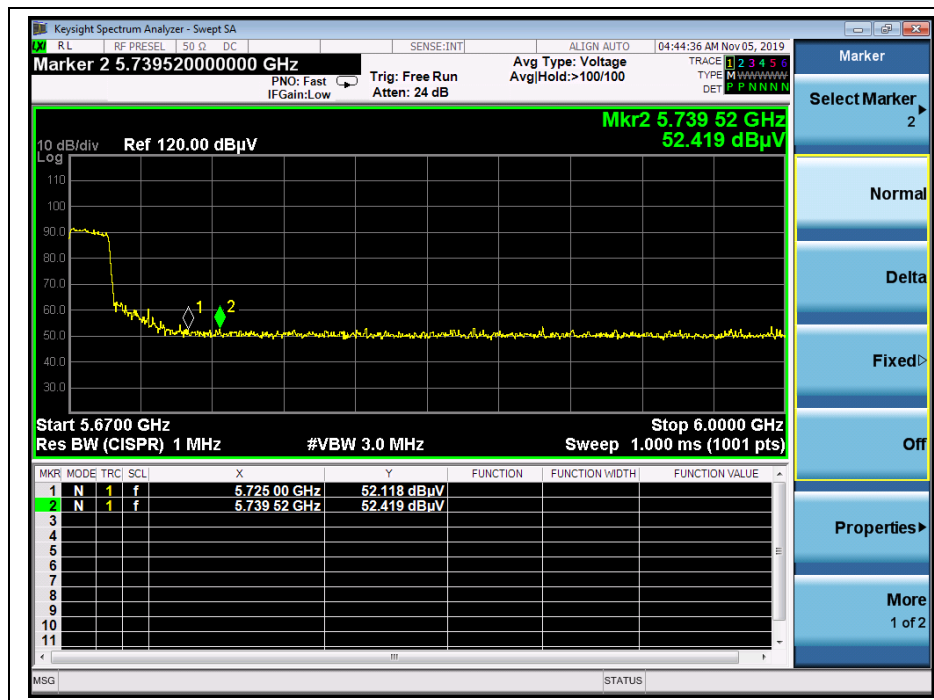
(Channel 142, PEAK, 802.11n (HT40))
