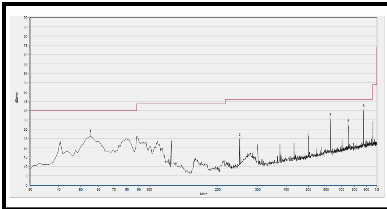
(Plot C: 30MHz – 1GHz, Test Antenna Vertical)
