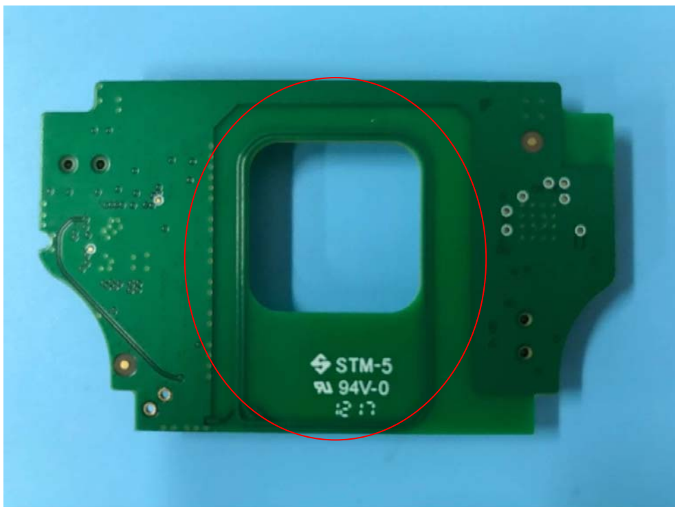
5. 13.56MHz antenna view
