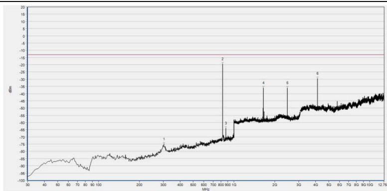
(Plot C1: EGPRS 850MHz Channel = 128, Test Antenna Horizontal)
