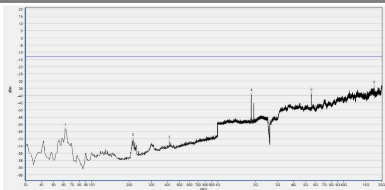
(Plot H1: HSDPA 1900MHz Channel = 9262, Test Antenna Horizontal)
