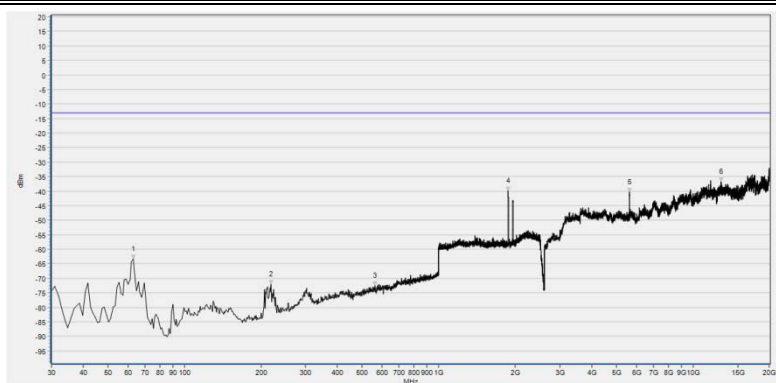
(Plot L3: HSPA+ 1900MHz Channel = 9400, Test Antenna Horizontal)
