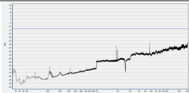
(Plot J5: HSUPA 1900MHz Channel = 9538, Test Antenna Horizontal)
