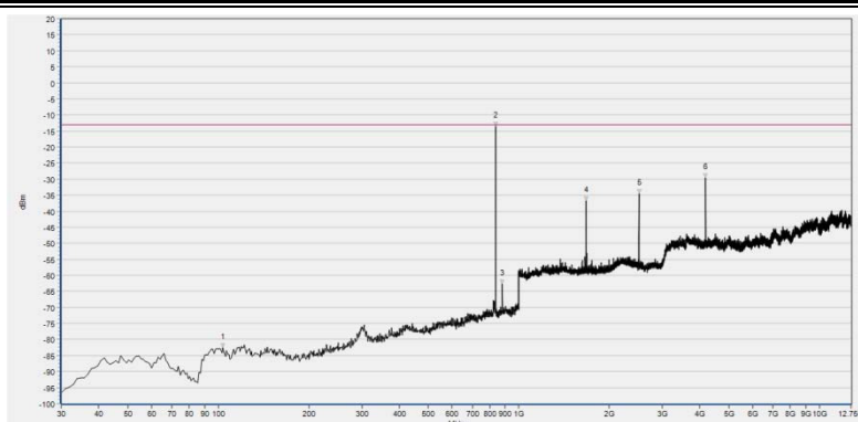
(Plot A3: GPRS 850MHz Channel = 190, Test Antenna Horizontal)
