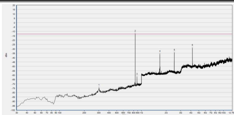
(Plot C3: EGPRS 850MHz Channel = 190, Test Antenna Horizontal)
