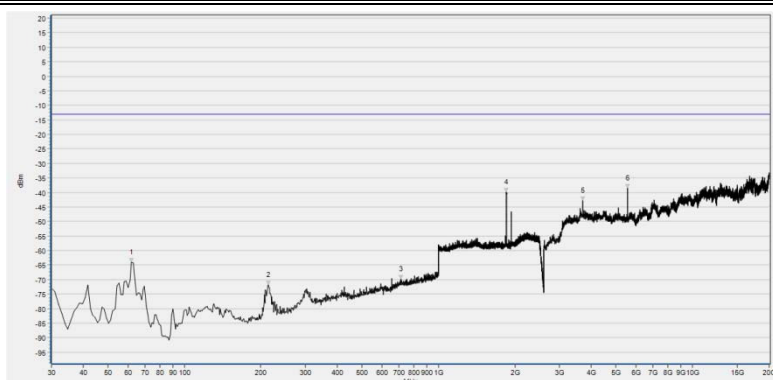
(Plot J1: HSUPA 1900MHz Channel = 9262, Test Antenna Horizontal)
