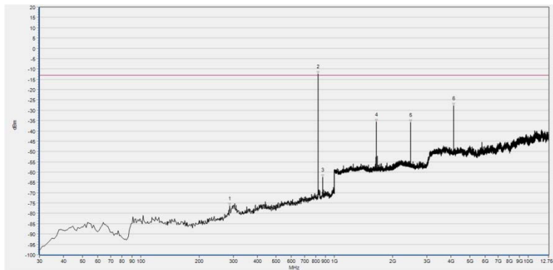
(Plot A1: GPRS 850MHz Channel = 128, Test Antenna Horizontal)
