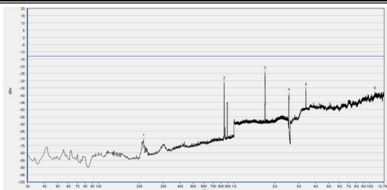
(Plot G5: HSDPA 850MHz Channel = 4233, Test Antenna Horizontal)
