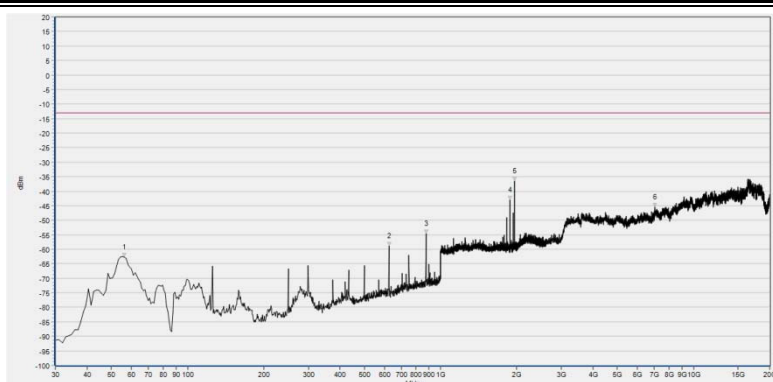
(Plot D3: EGPRS 1900MHz Channel = 661, Test Antenna Horizontal)
