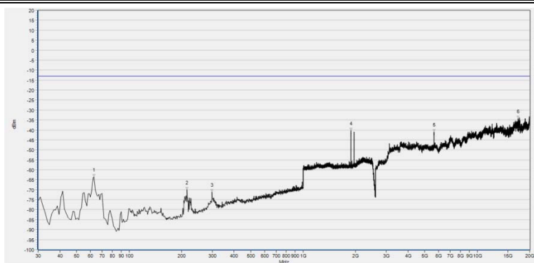
(Plot H3: HSDPA 1900MHz Channel = 9400, Test Antenna Horizontal)
