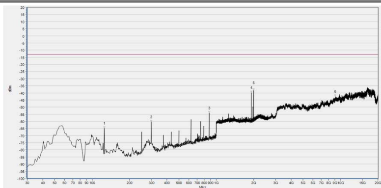
(Plot D5: EGPRS 1900MHz Channel = 810, Test Antenna Horizontal)
