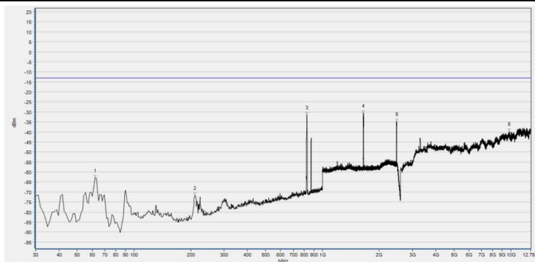
(Plot I1: HSUPA 850MHz Channel = 4132, Test Antenna Horizontal)
