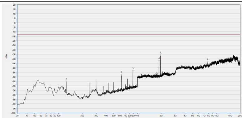
(Plot B3: GPRS 1900MHz Channel = 661, Test Antenna Horizontal)
