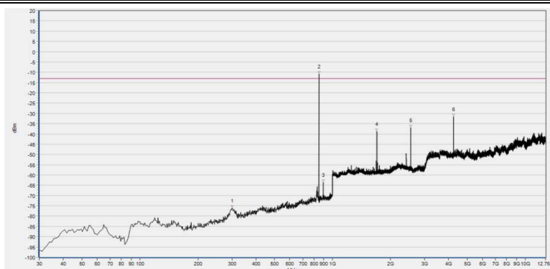
(Plot C5: EGPRS 850MHz Channel = 251, Test Antenna Horizontal)
