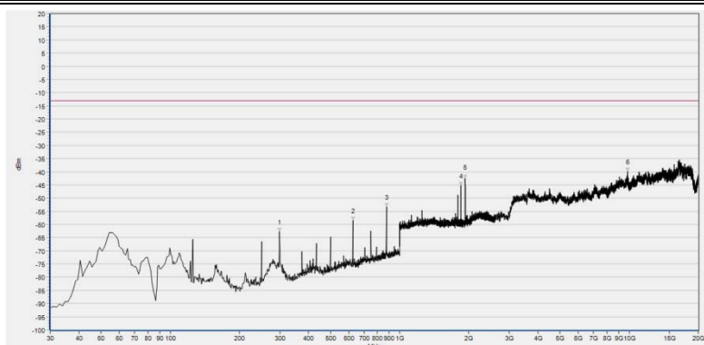
(Plot B1: GPRS 1900MHz Channel = 512, Test Antenna Horizontal)
