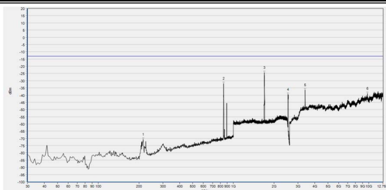
(Plot I5: HSUPA 850MHz Channel = 4233, Test Antenna Horizontal)
