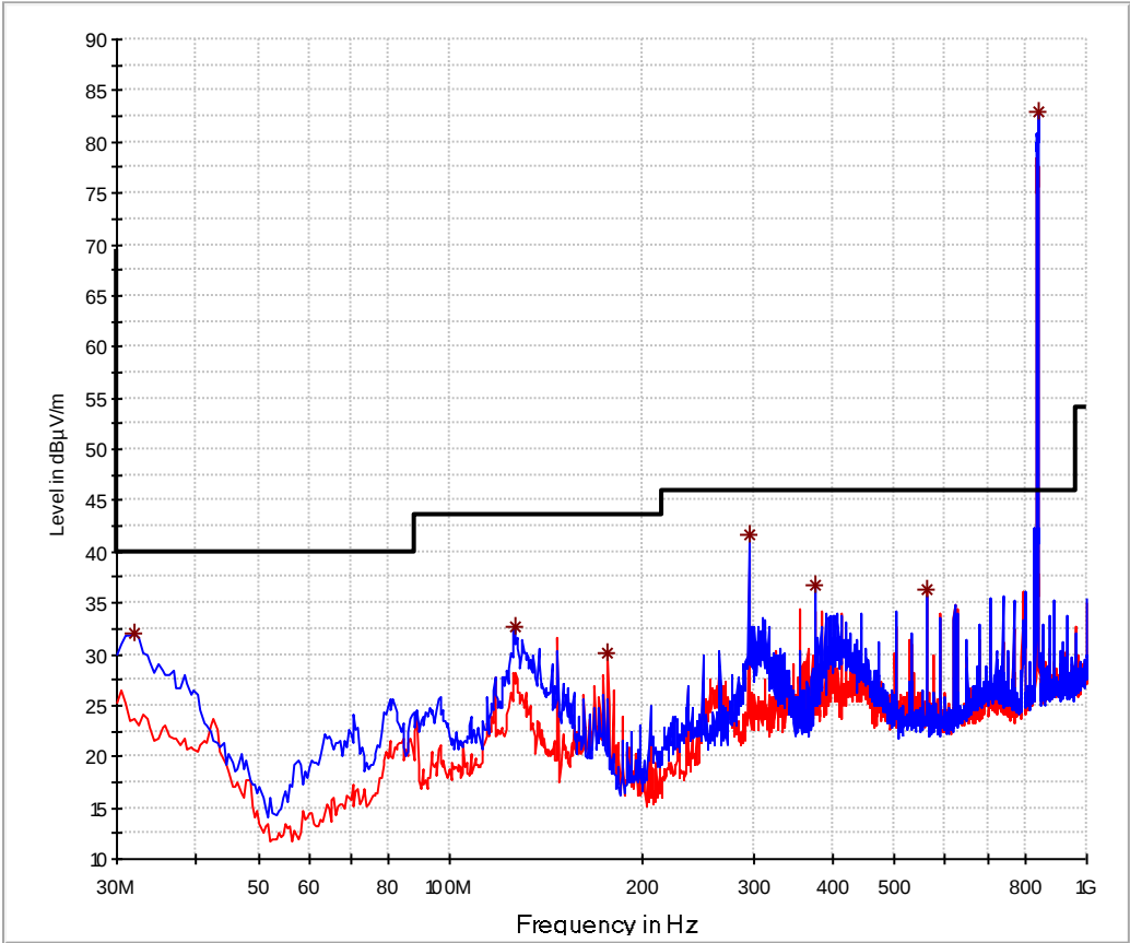
Preview Result 1H-PK+ Preview Result 1V-PK+ FCC 15.209 * Final_Result P
