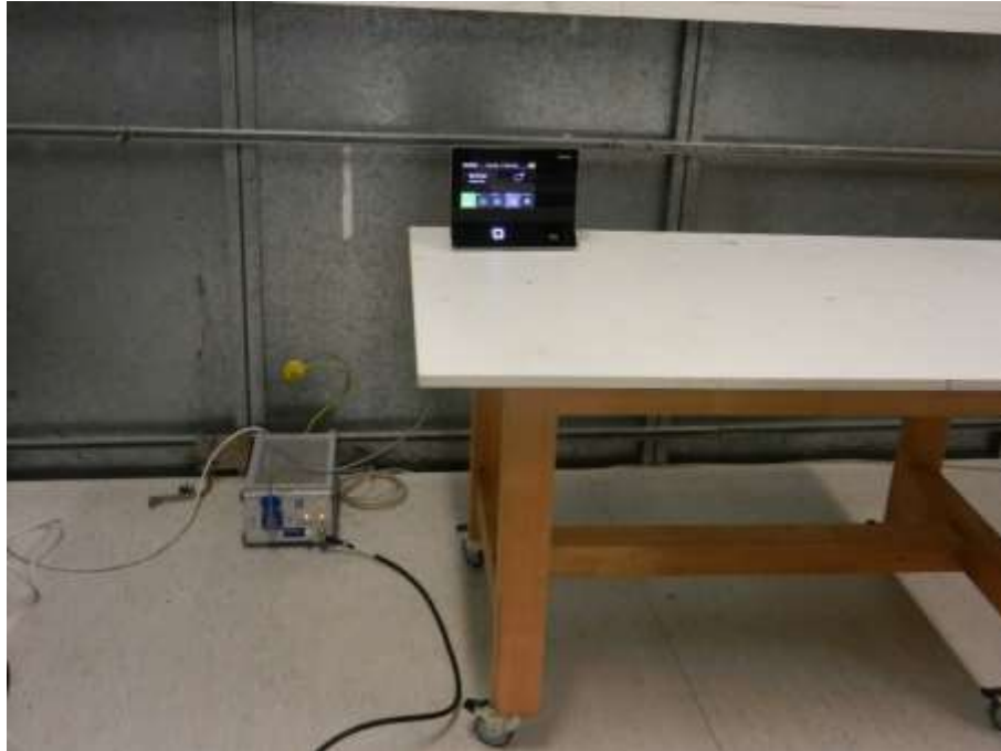
Figure 1: Conducted AC Emissions
