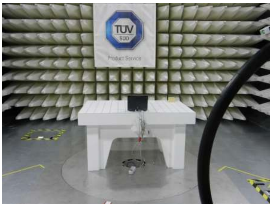
Figure 2: Radiated Emissions 9 kHz - 30 MHz
