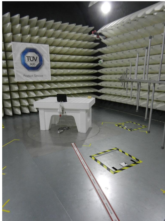
Figure 3 Radiated Emissions 30 MHz - 1 GHz
