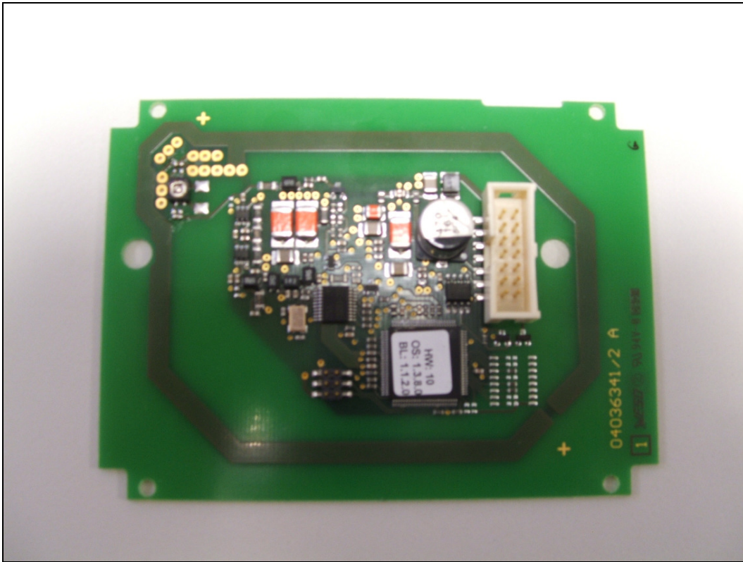
LEGIC advant PCB inclusive antenna (front)
