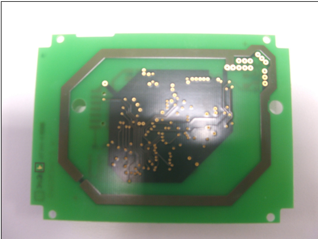
LEGIC advant PCB inclusive antenna (back)
