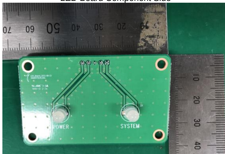
LED Board Component Side
