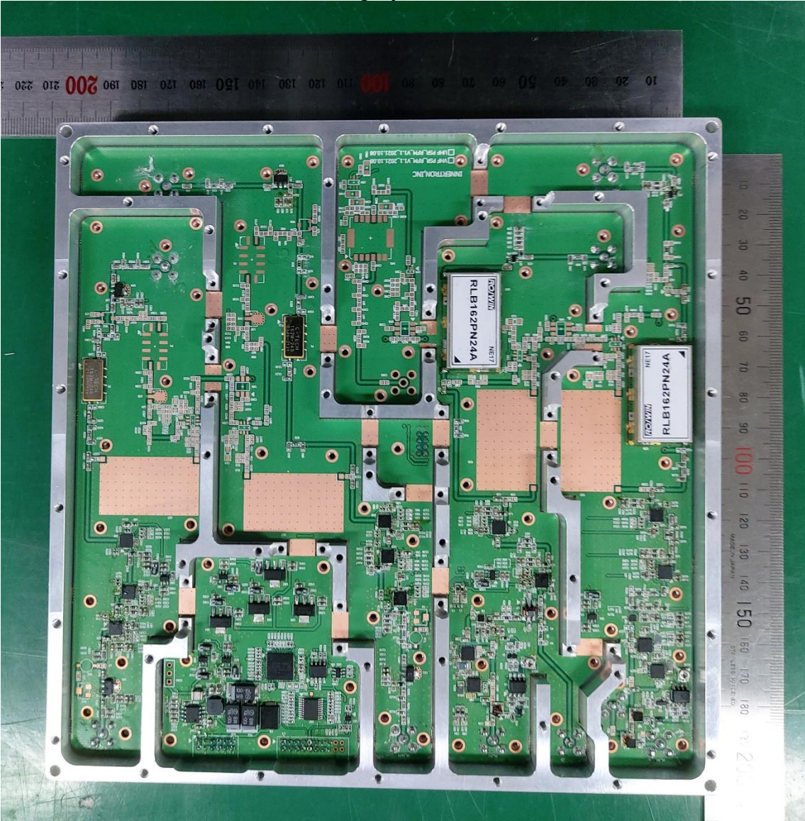
Photograph of UDCU
