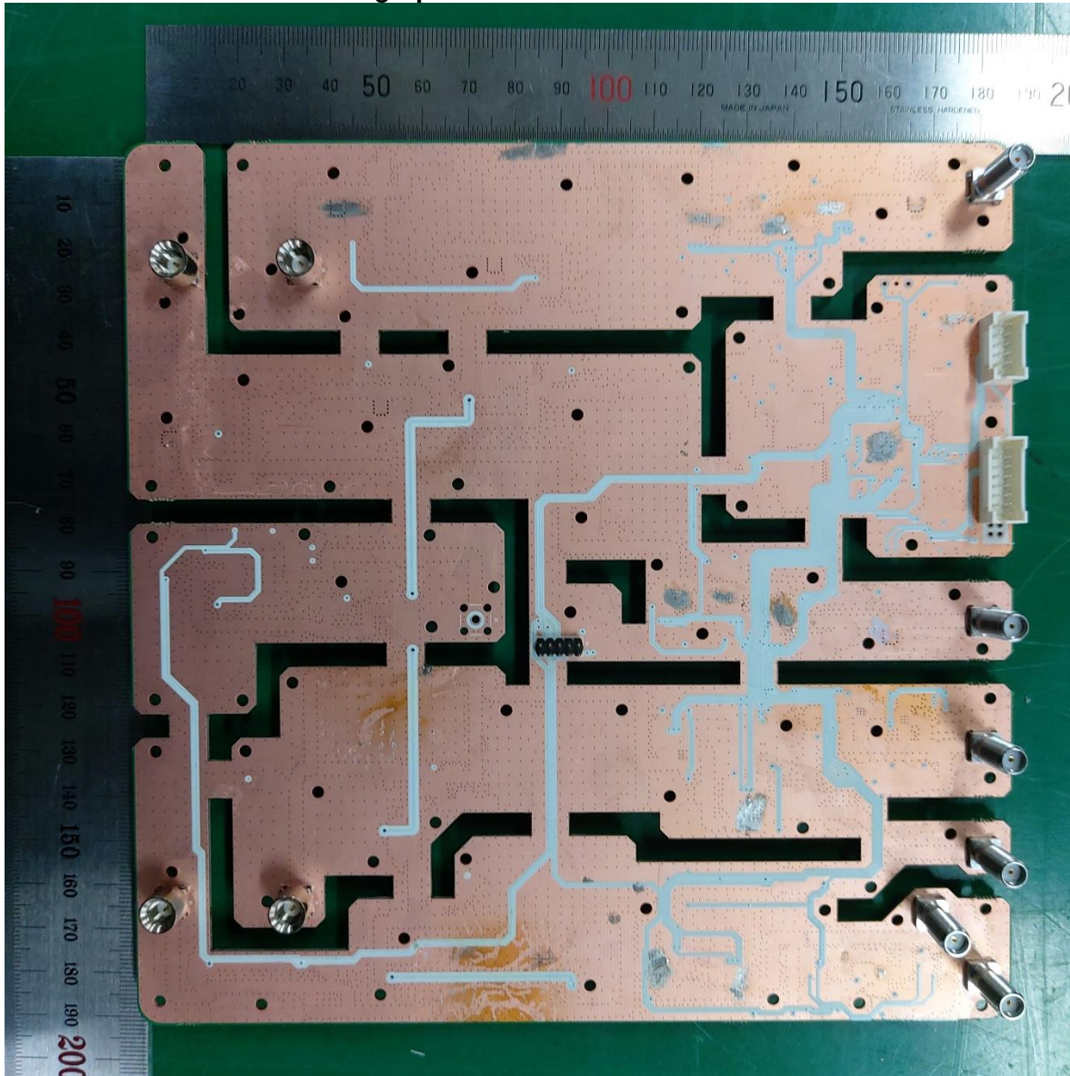
Photograph of UDCU Board: Foil Side
