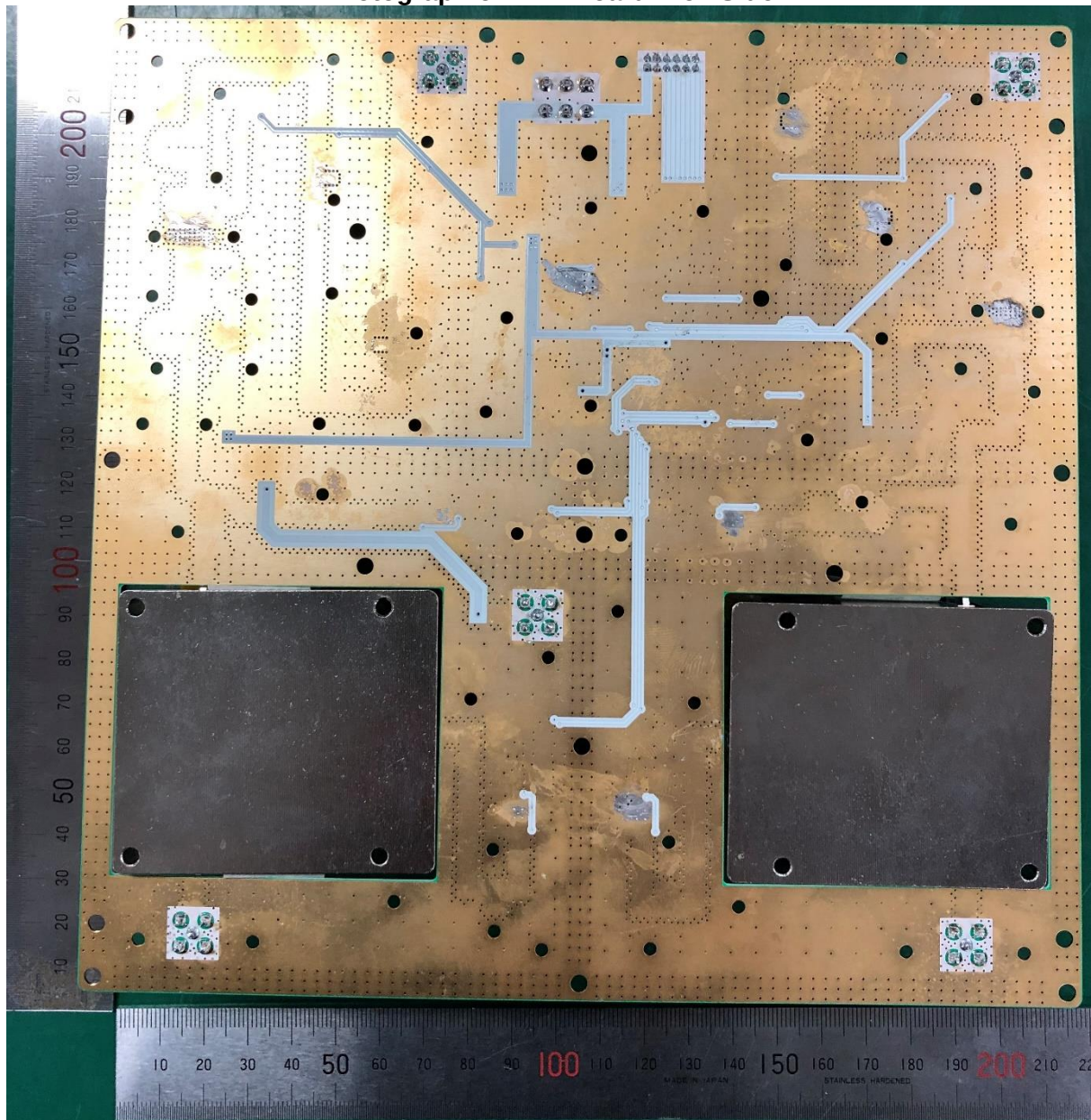
Photograph of HPA Board: Foil Side
