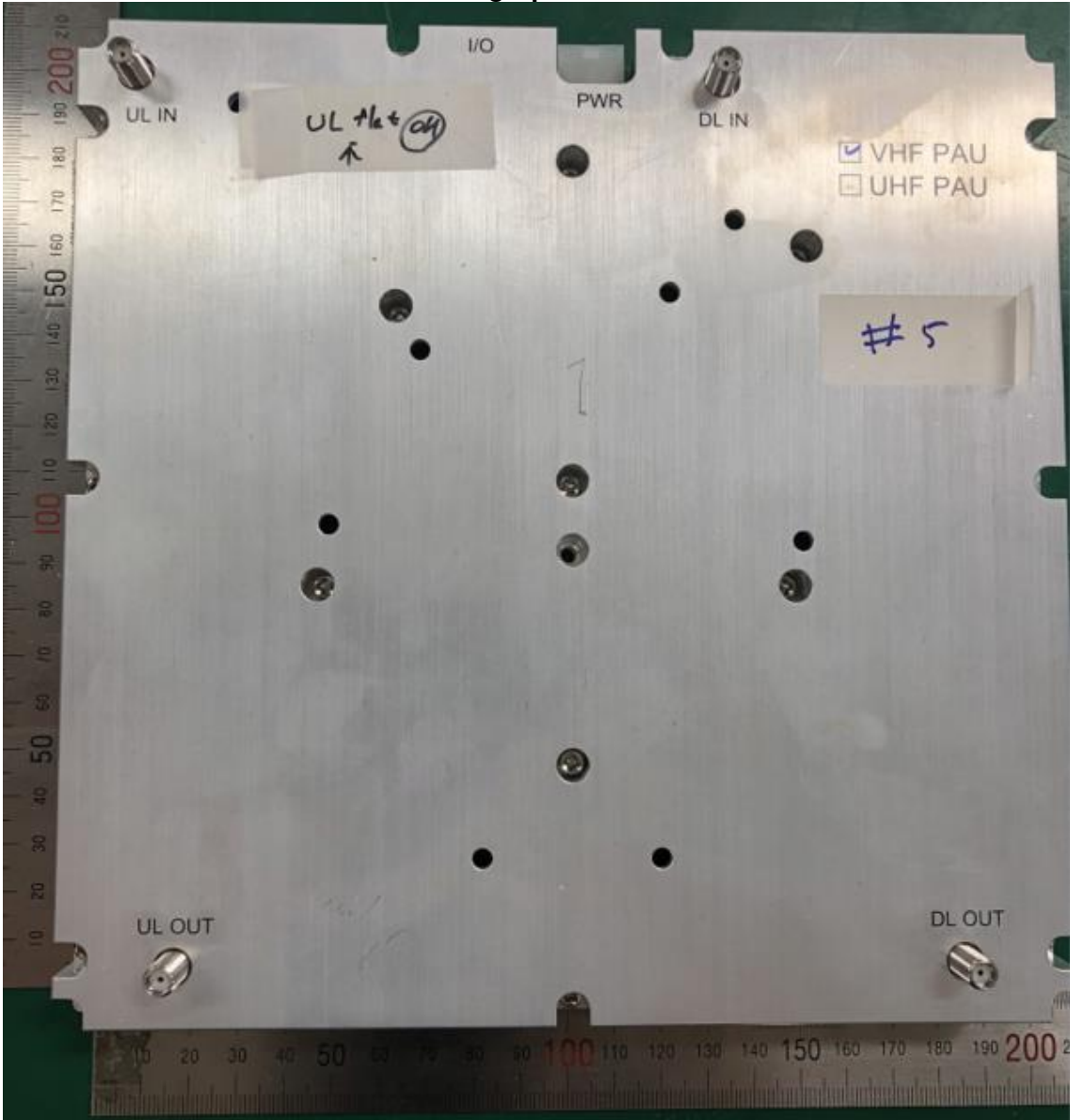
Photograph of HPA
