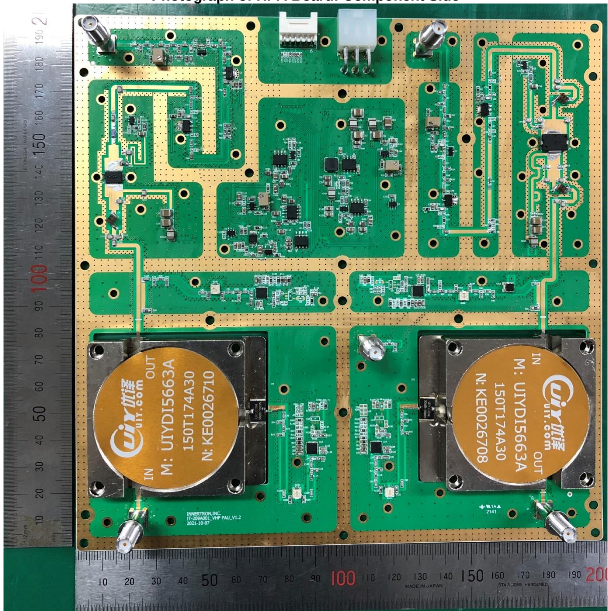
Photograph of HPA Board: Component Side
