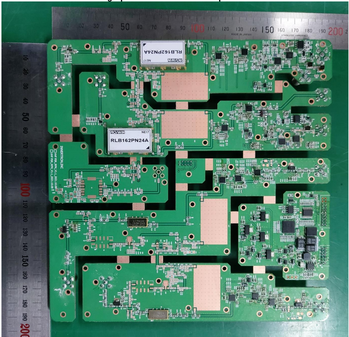
Photograph of UDCU Board: Component Side
