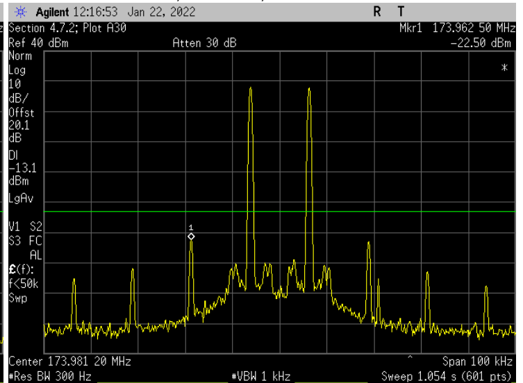
25 kHz Delta; 174 MHz; AGC+3dB
