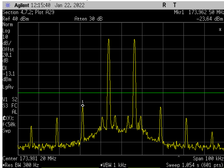
25 kHz Delta; 174 MHz; Below AGC
