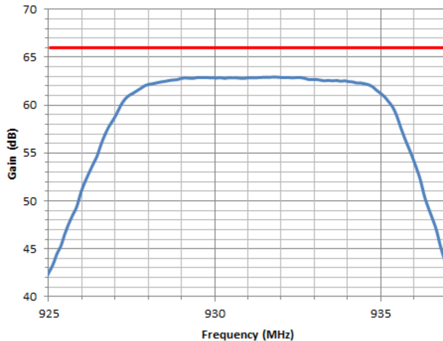
Gain vs. Frequency
