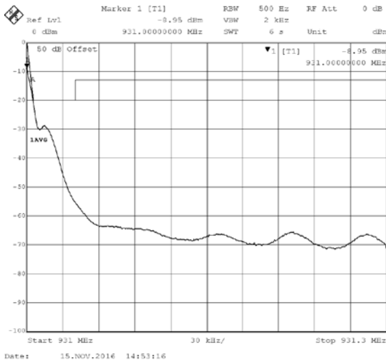
930-931 MHz high band edge emissions, single test signal, input level below (left) and above (right) AGC threshold
