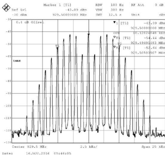
929.5 MHz 11K3F3E input (left) and output (right), level above AGC threshold
