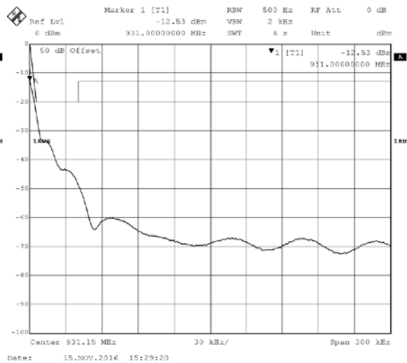
930-931 MHz high band edge emissions, two adjacent test signals, input level below (left) and above (right) AGC threshold
