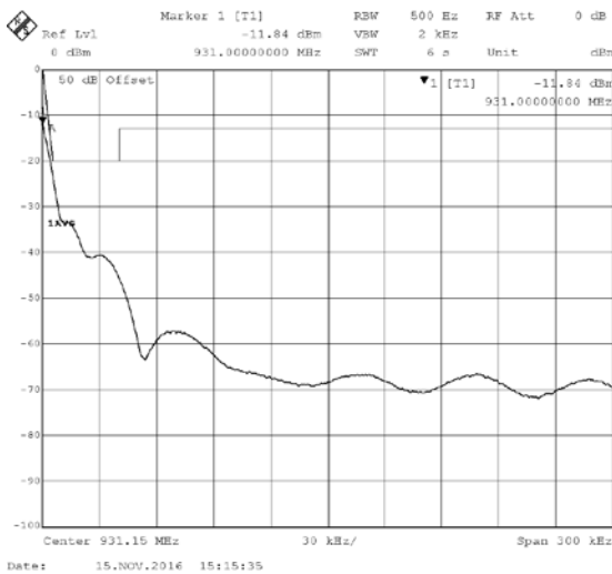
930-931 MHz high band edge emissions, two adjacent test signals, input level below (left) and above (right) AGC threshold
