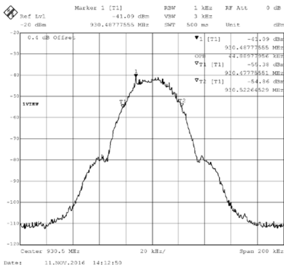
930.5 MHz 2-GFSK input (left) and output (right), level below AGC threshold
