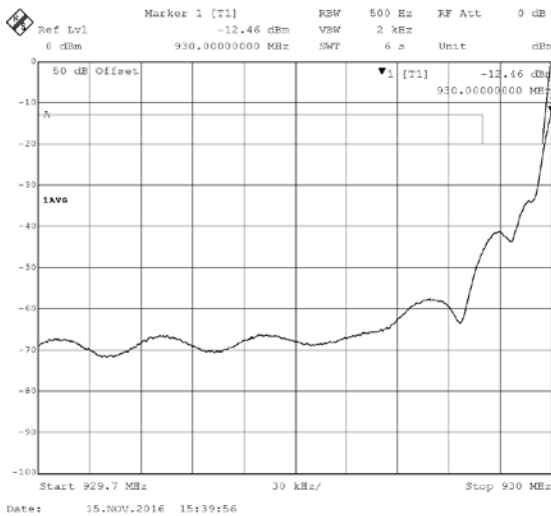
930-931 MHz low band edge emissions, two adjacent test signals, input level below (left) and above (right) AGC threshold
