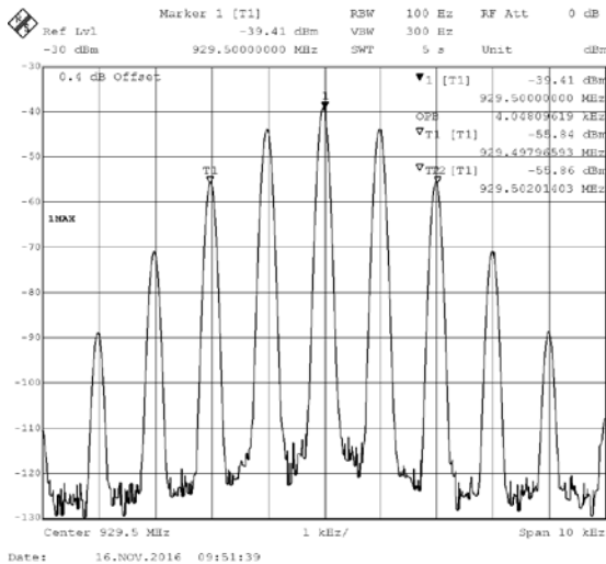
929.5 MHz 4K00F3E input (left) and output (right), level below AGC threshold
