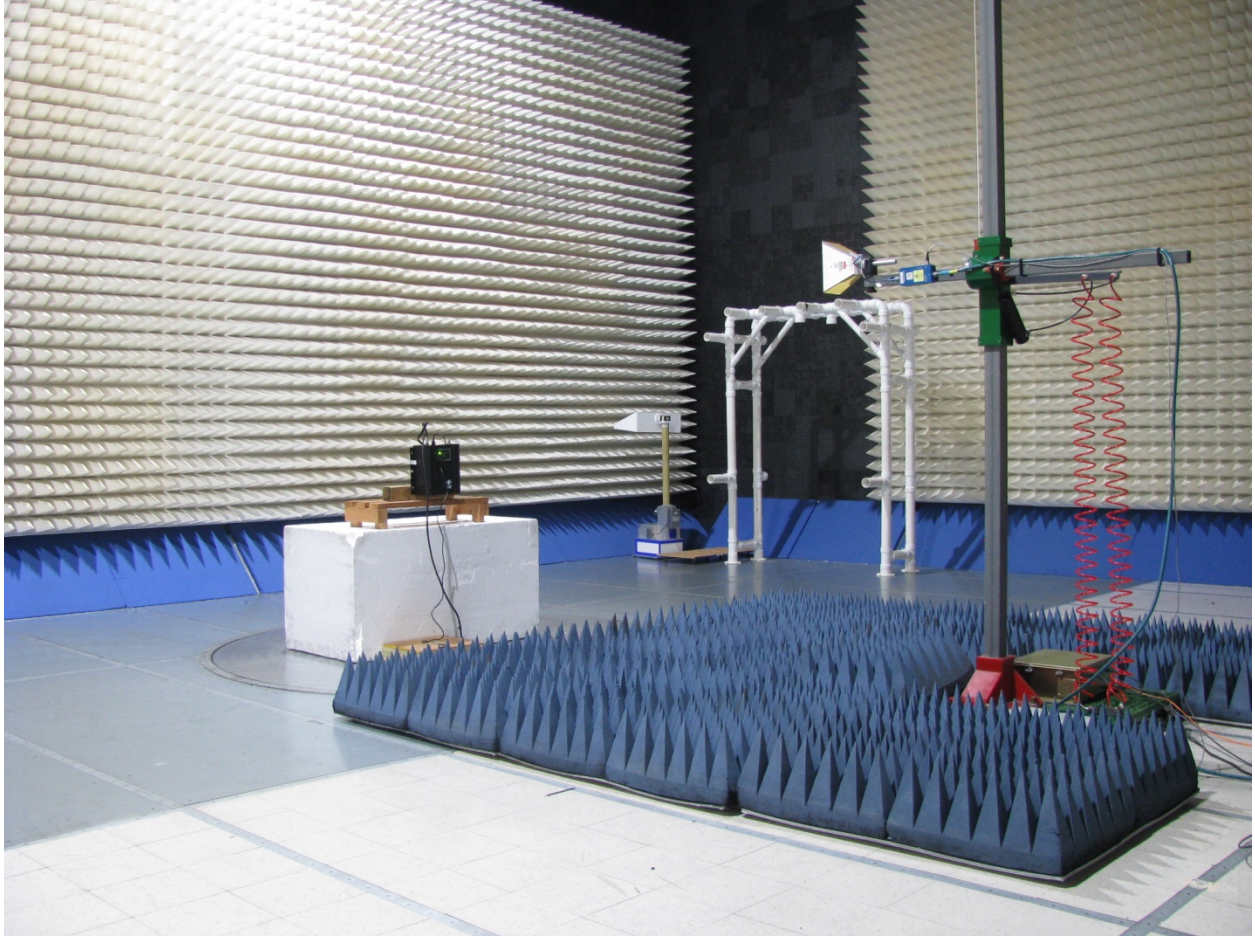
Radiated spurious emissions (1)
