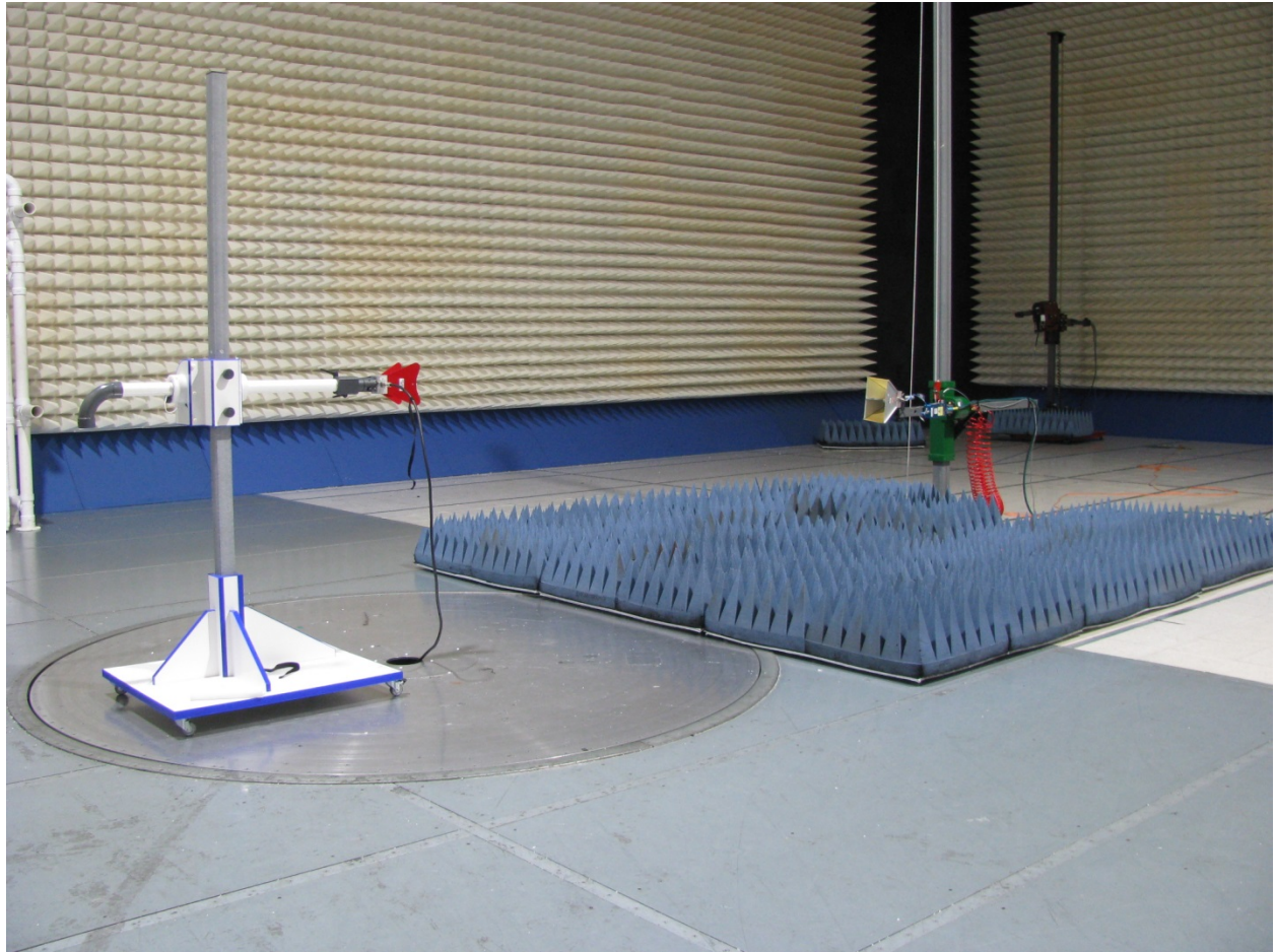
Radiated spurious emissions (2)
