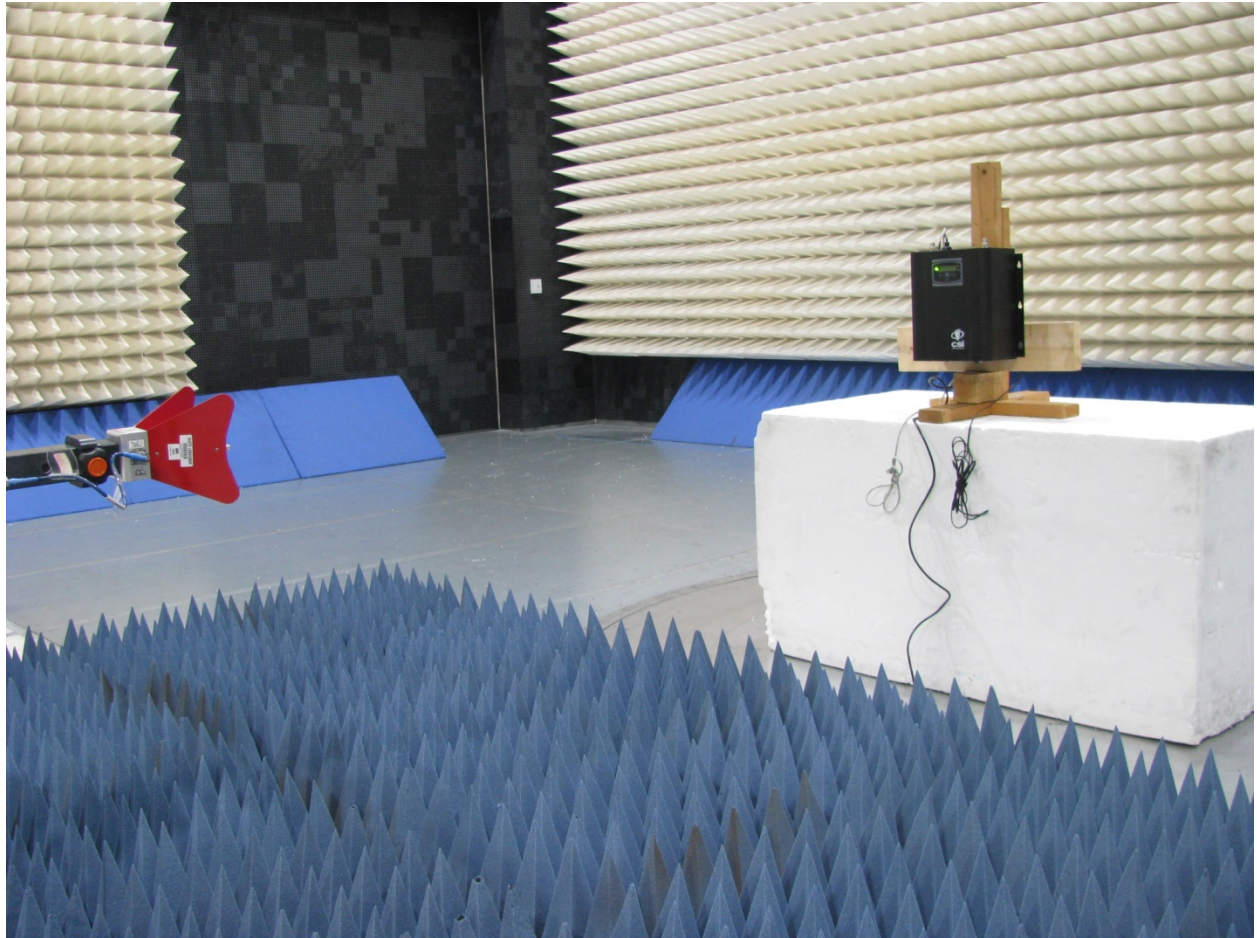
Radiated emissions
